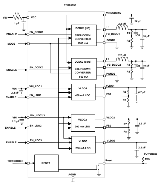
Typical Application Schematic
