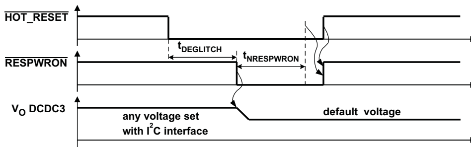
Figure 1. HOT_RESET Timing
