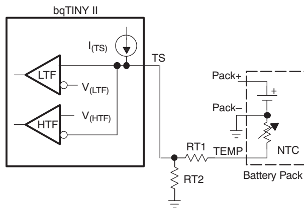
Figure 28. TS Pin Threshold
