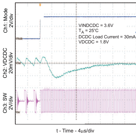
Figure 13. PFM to PWM Transition (DC-DC)
