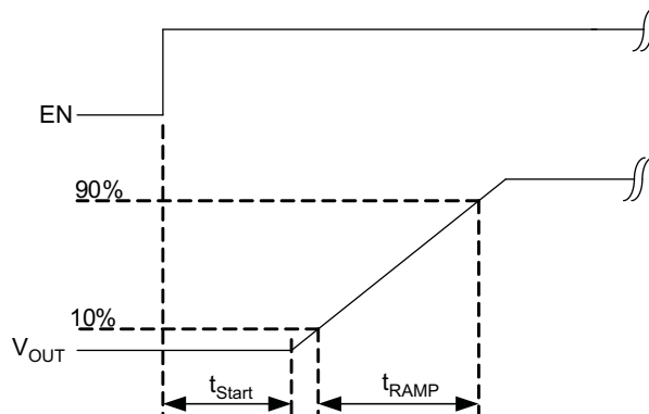
Figure 18. Soft Start
