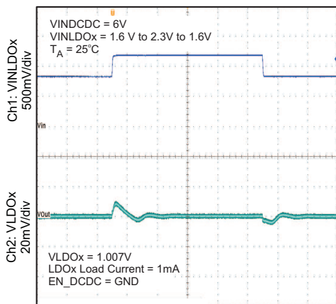
Figure 26. Line Transient Response (LDOx)
