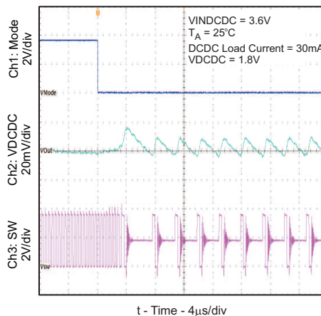
Figure 14. PWM to PFM Transition (DC-DC)
