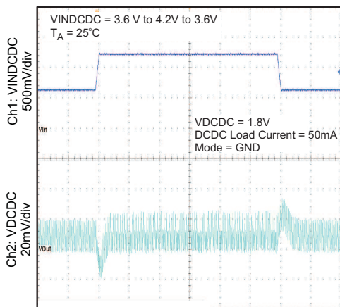
Figure 24. Line Transient Response (DC-DC PFM Mode)
