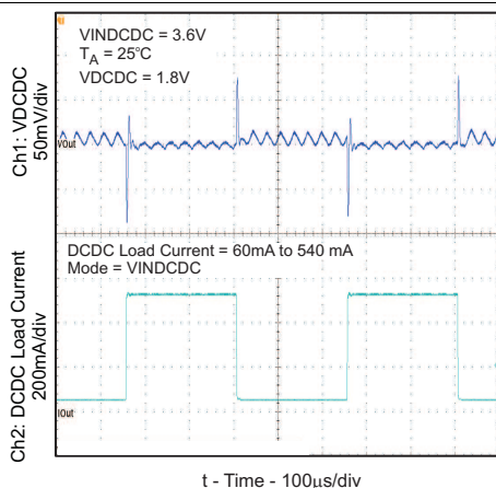
Figure 11. Load Transient Response (DC-DC PWM Mode)
