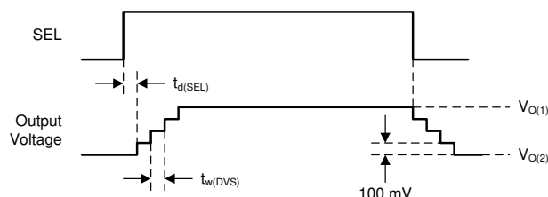
Figure 7-10. Dynamic Voltage Scaling with High Load
