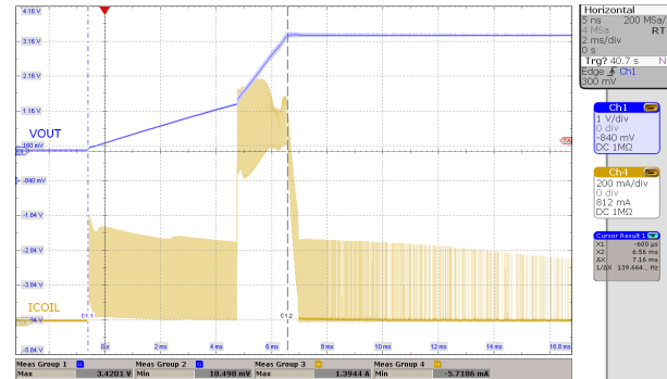
Figure 8-31. Start-up Behavior from Rising Enable
