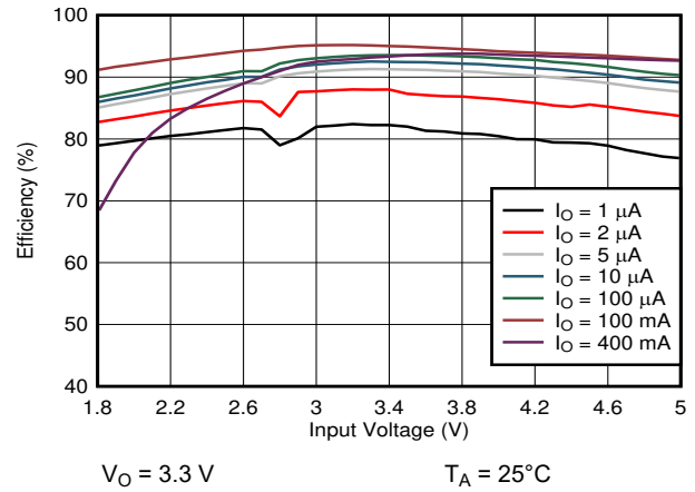
Figure 8-9. Efficiency versus Input Voltage
