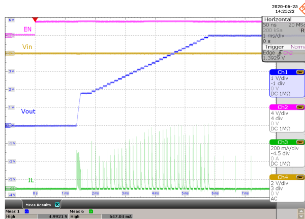
Figure 8-28. Start-up Behavior from Rising Enable
