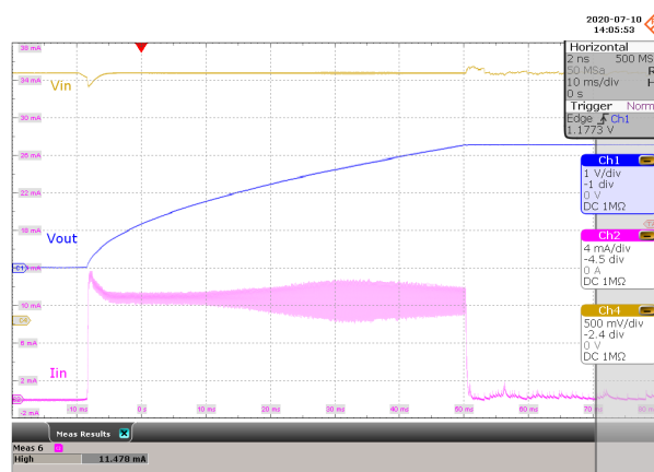
Figure 8-33. Start-up with 2.5-mA ICL
