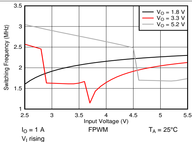
Figure 53. Switching Frequency versus Input Voltage
