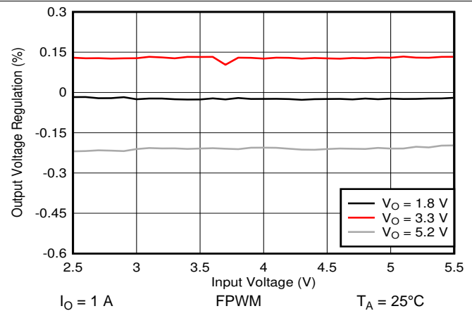
Figure 35. Line Regulation
