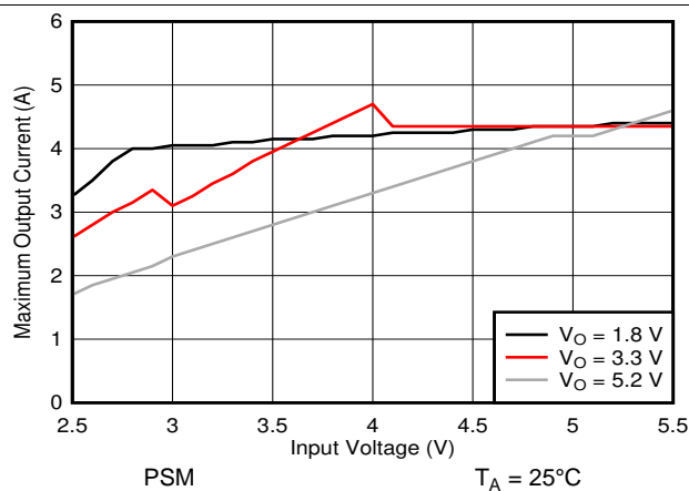
Figure 55. Maximum Output Current versus Input Voltage
