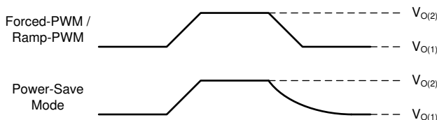
Figure 14. Ramp-PWM Operation
