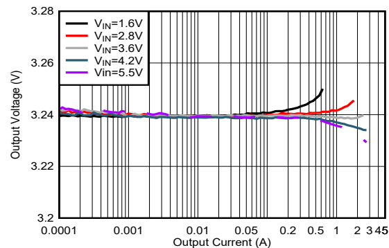
Figure 8-4. Load Regulation (FPWM)
