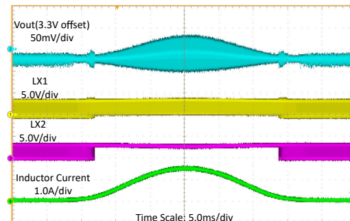
Figure 8-15. Load Sweep at 2.7-V Input Voltage
