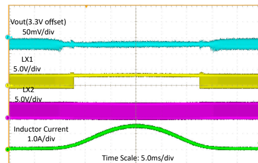
Figure 8-19. Load Sweep at 4.3-V Input Voltage
