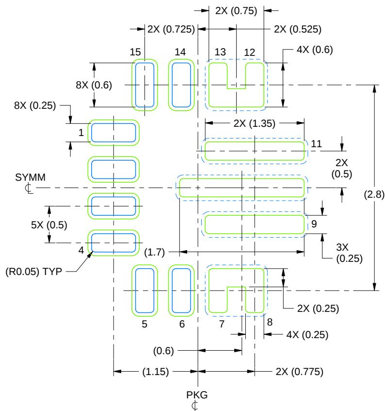
LAND PATTERN EXAMPLE
