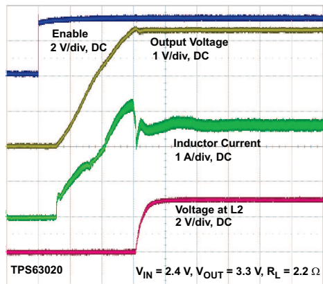
Time 400 \mu s/div Figure 26. Start-up Behavior from Rising Enable, TPS63020
