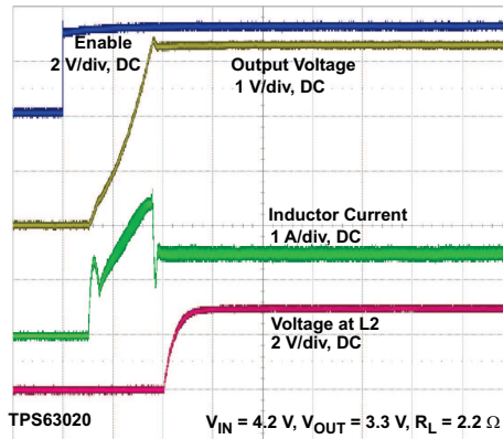
Time 100 \mu s/div Figure 27. Start-up Behavior from Rising Enable, TPS63020
