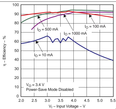
Figure 20. Efficiency vs Input Voltage (TPS63012)
