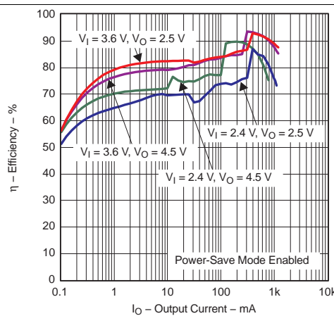
Figure 4. Efficiency vs Output Current (TPS63010)
