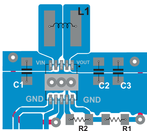
Figure 20. Layout Recommendation
