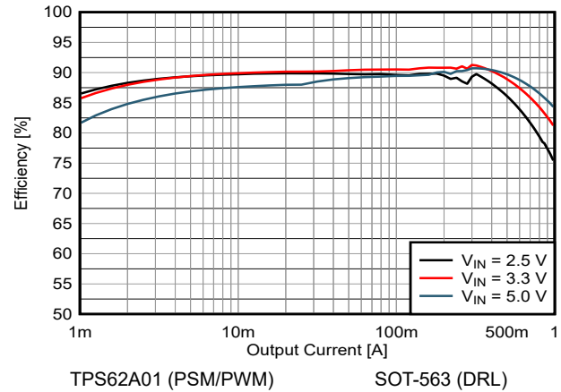
Figure 8-5. 1.2V Output Efficiency
