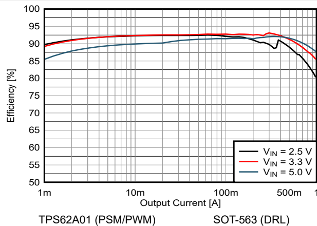
Figure 8-6. 1.8V Output Efficiency
