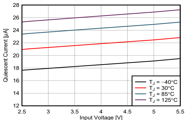
Figure 6-2. Quiescent Current vs Input Voltage (TPS62A02)
