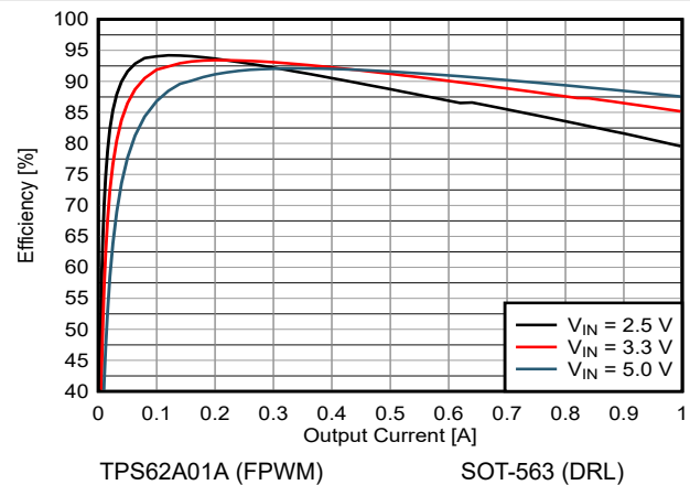
Figure 8-7. 1.8V Output Efficiency
