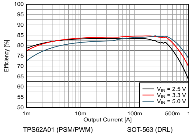
Figure 8-4. 0.6V Output Efficiency
