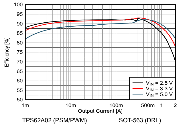
Figure 8-9. 1.2V Output Efficiency
