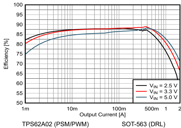
Figure 8-8. 0.6V Output Efficiency
