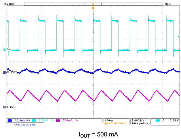
Figure 8-11. PWM Operation
