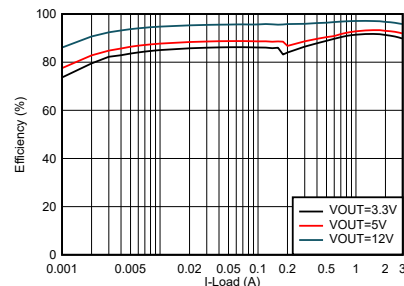
TPS62933 Efficiency, V_{IN} = 24 V, f_{SW} = 500 kHz
