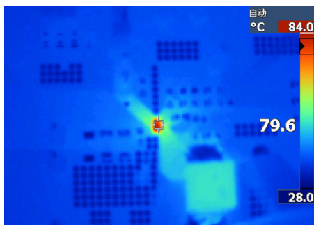
Figure 10-8. Case Temperature, V_{IN} = 24\text{ V} , I_{OUT} = 3\text{ A} , f_{SW} = 500\text{ kHz}
