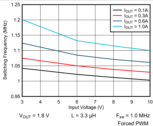
Figure 9-35. Switching Frequency vs Input Voltage
