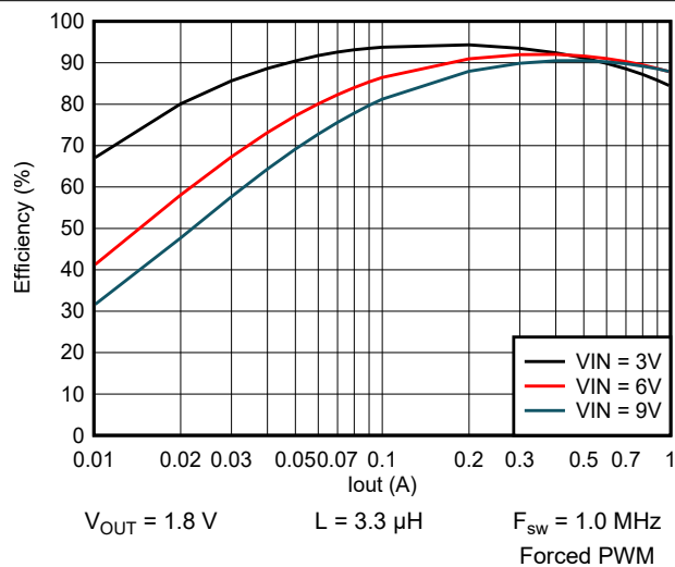
Figure 9-33. Efficiency vs Output Current
