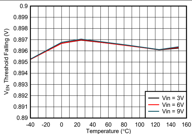
Figure 7-18. Precision Enable Threshold vs Temperature
