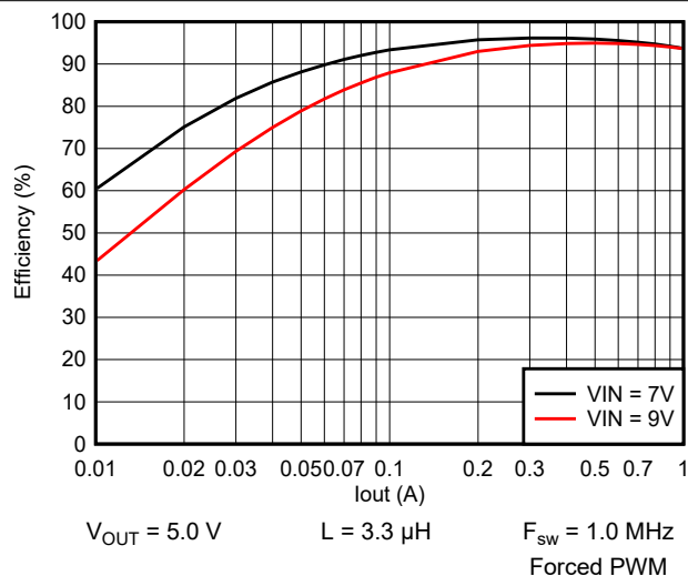
Figure 9-9. Efficiency vs Output Current
