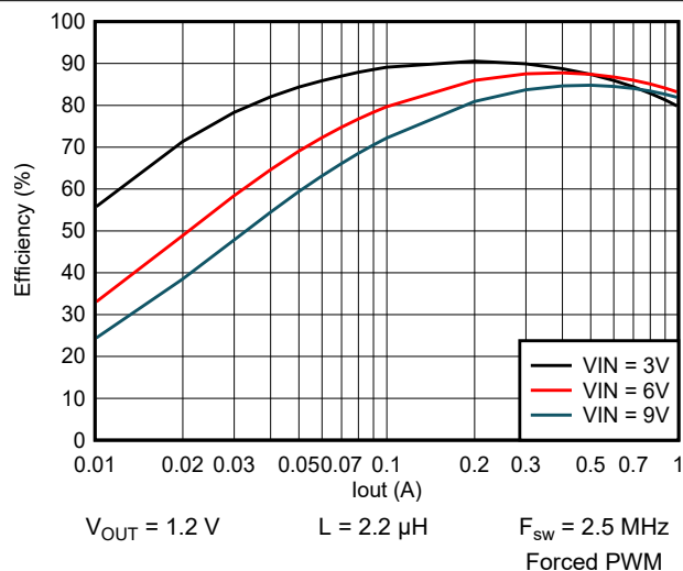
Figure 9-39. Efficiency vs Output Current
