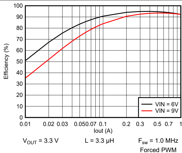
Figure 9-21. Efficiency vs Output Current
