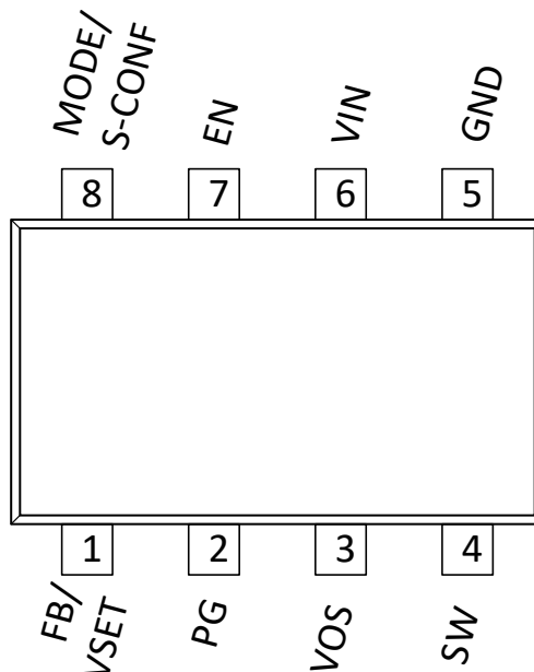
Figure 6-1. TPS629210E 8-Pin DRL SOT-5X3 Pinout
