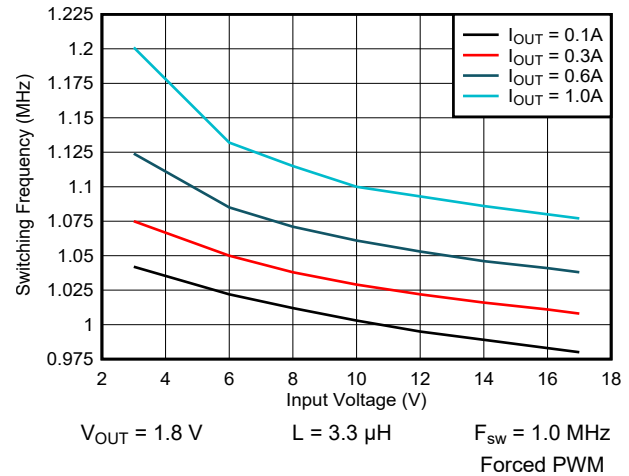
Figure 9-35. Switching Frequency vs Input Voltage
