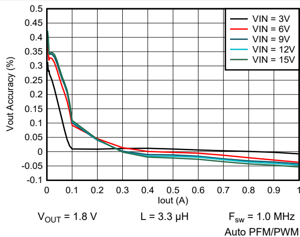
Figure 9-36. Output Voltage vs Output Current
