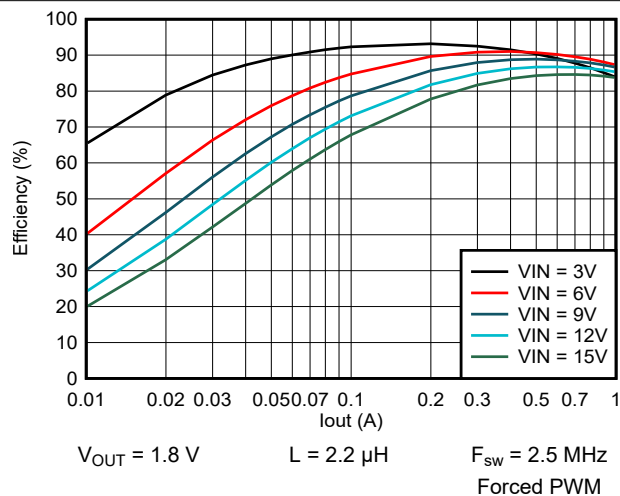
Figure 9-27. Efficiency vs Output Current
