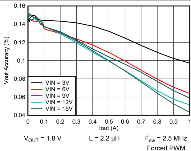
Figure 9-31. Output Voltage vs Output Current
