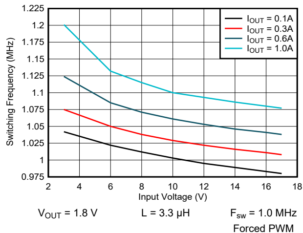
Figure 9-35. Switching Frequency vs Input Voltage
