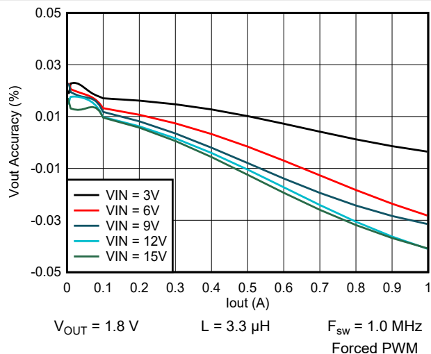
Figure 9-37. Output Voltage vs Output Current
