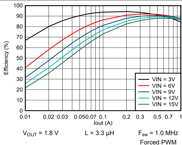
Figure 9-33. Efficiency vs Output Current
