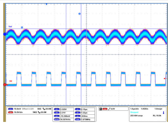
Figure 9-75. Output Voltage Ripple
