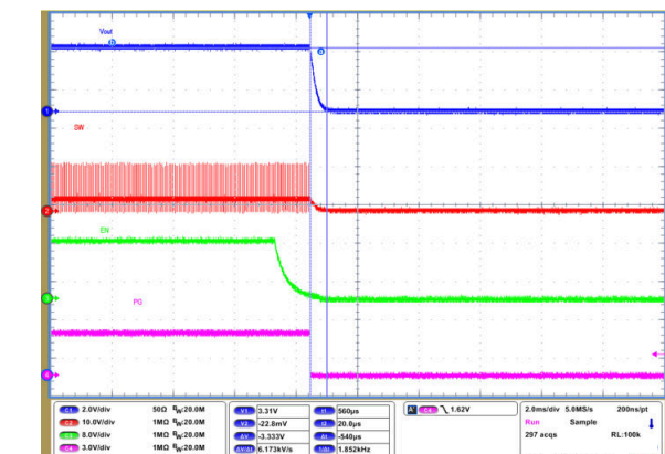
Figure 9-65. Shutdown Timing with Output Discharge Enabled
