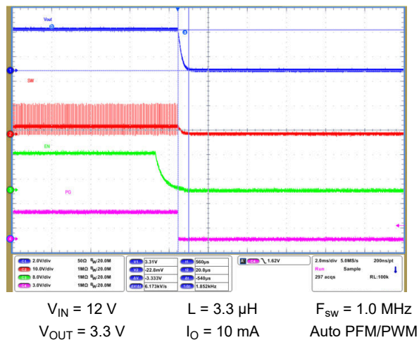
Figure 9-66. Shutdown Timing with Output Discharge Enabled
