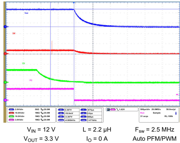
Figure 9-65. Shutdown Timing with Output Discharge Enabled
