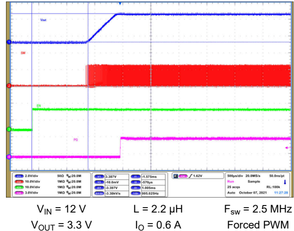
Figure 9-63. Start-Up Timing
