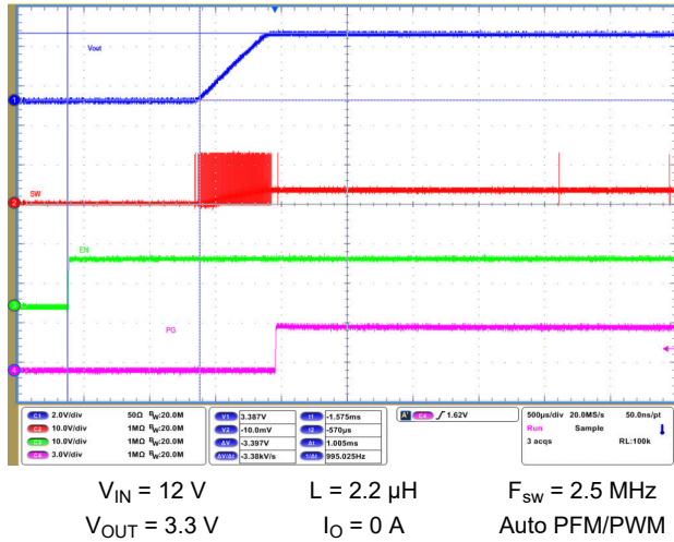
Figure 9-62. Start-Up Timing
