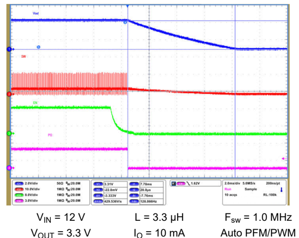
Figure 9-67. Shutdown Timing with Output Discharge Disabled
