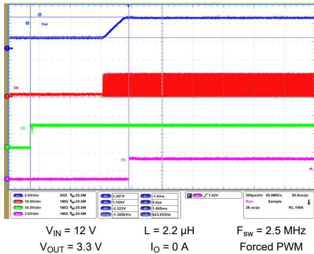
Figure 9-64. Start-Up into Prebiased Output
