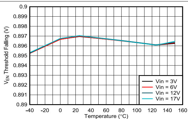
Figure 7-18. Precision Enable Threshold vs Temperature
