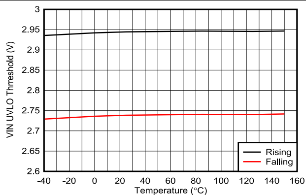
Figure 7-16. V_{IN} UVLO Thresholds vs Temperature
