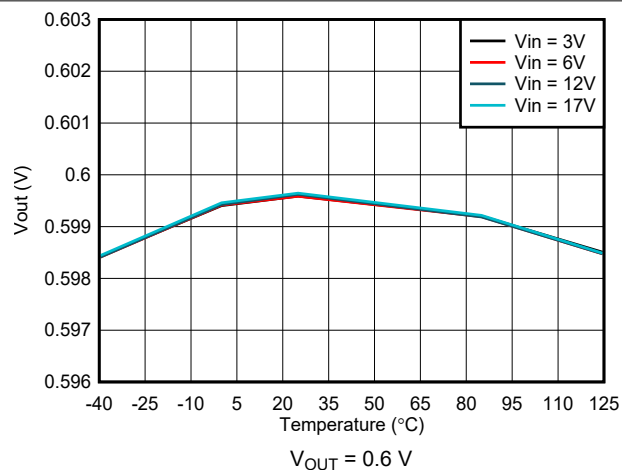
Figure 7-8. Output Voltage Accuracy – VSET Selected
