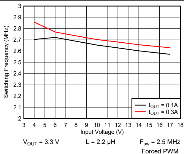
Figure 9-17. Switching Frequency vs Input Voltage
