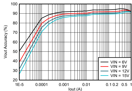
Efficiency vs Output Current V_{OUT} = 3.3 \text{ V} at 1.0-MHz Auto PFM/PWM
