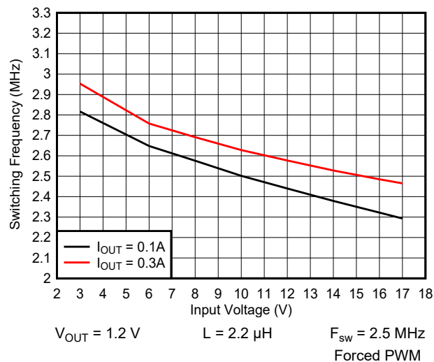
Figure 9-41. Switching Frequency vs Input Voltage
