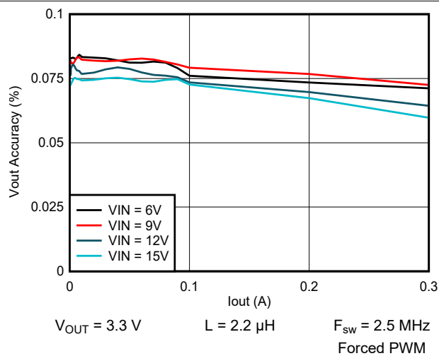
Figure 9-19. Output Voltage vs Output Current
