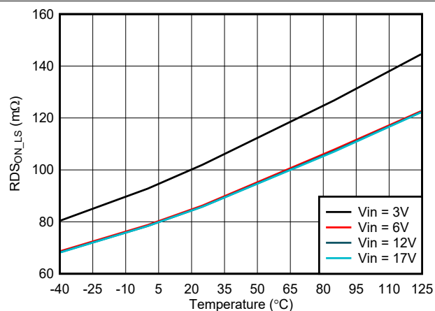
Figure 7-12. Low-Side R_{DS(on)} vs Temperature
