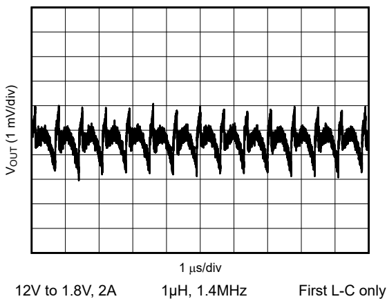
Figure 5-5. V_{OUT} Ripple After the First L-C Filter
