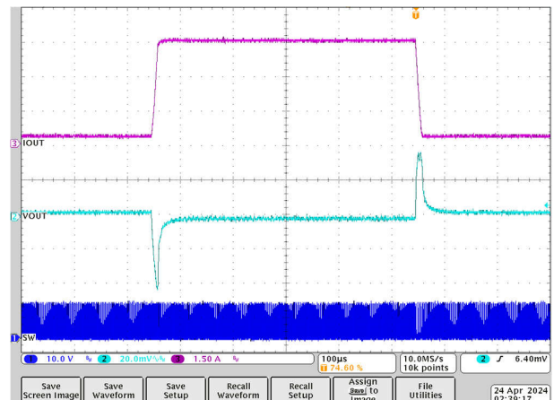
300mA to 4.5A to 300mA 12V to 1.2V 1µH, 1MHz After 2nd L-C
