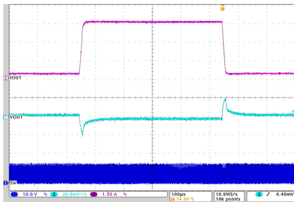
300mA to 4.5A to 300mA 12V to 1.8V 1µH, 1MHz 1st L-C only
