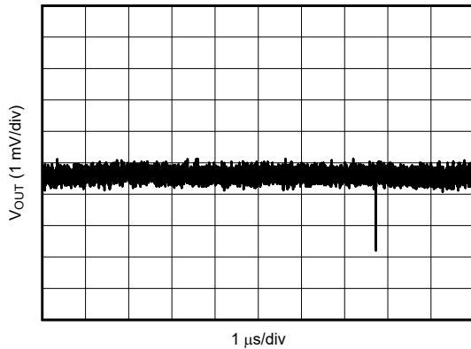
Figure 5-7. V_{OUT} Ripple After the Second L-C Filter
