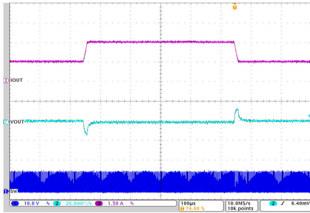
1.5A to 3A to 1.5A 12V to 1.2V 1µH, 1MHz After 2nd L-C
