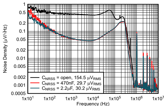
Output Noise vs Frequency
