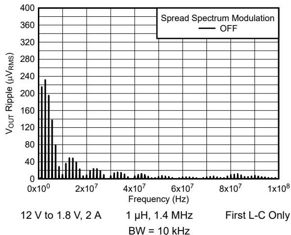
Figure 5-6. V_{OUT} Ripple FFT After the First L-C Filter
