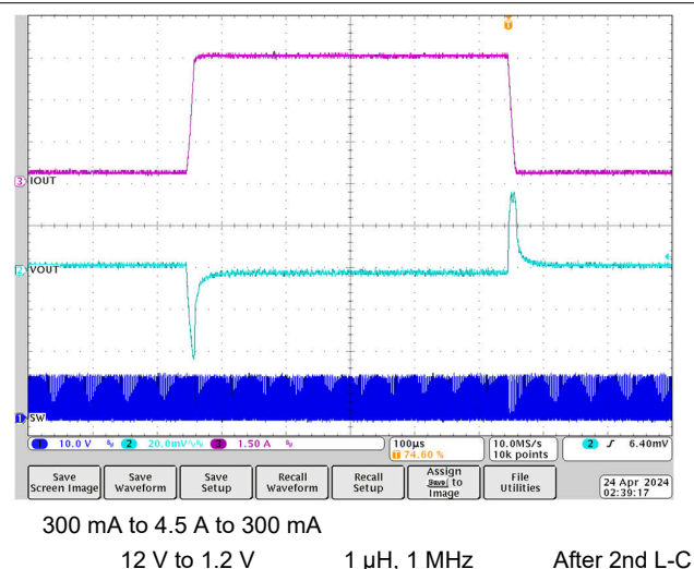
Figure 7-13. Load Transient
