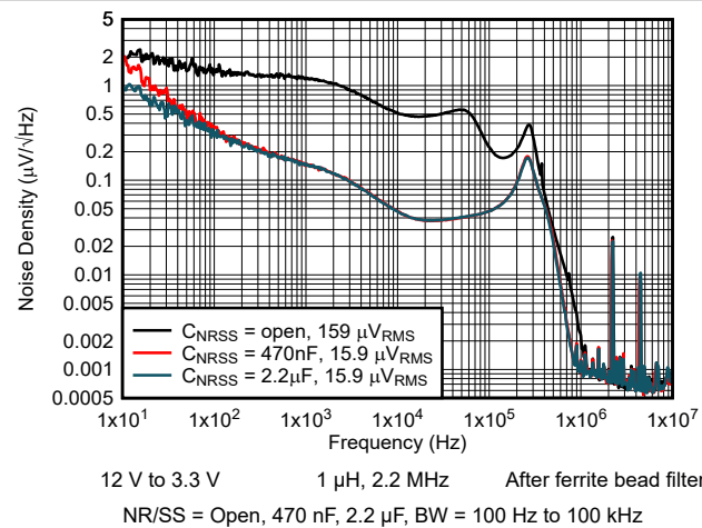
Figure 5-18. Output Noise Density vs Frequency
