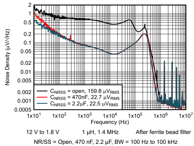
Figure 5-16. Output Noise Density vs Frequency
