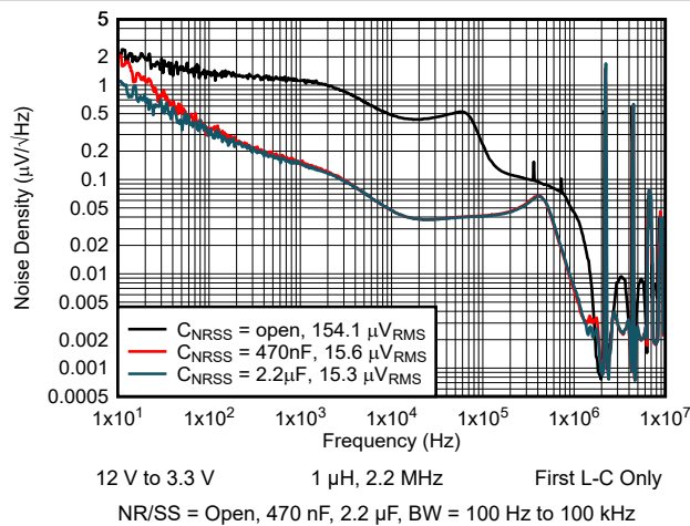
Figure 5-17. Output Noise Density vs Frequency
