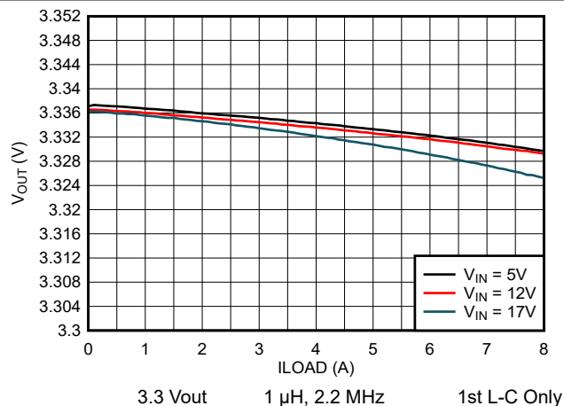
Figure 7-9. Output Voltage vs Load Current
