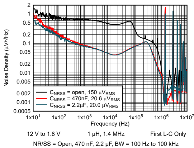
Figure 5-15. Output Noise Density vs Frequency
