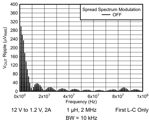
Figure 5-2. V_{OUT} Ripple FFT After the First L-C Filter
