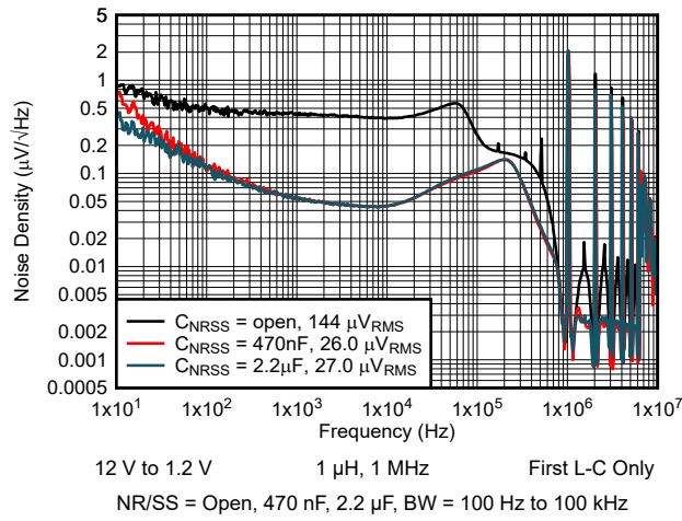
Figure 5-13. Output Noise Density vs Frequency
