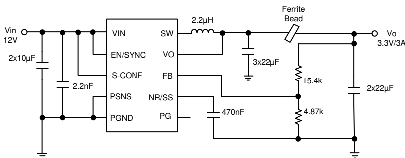
Typical Application
