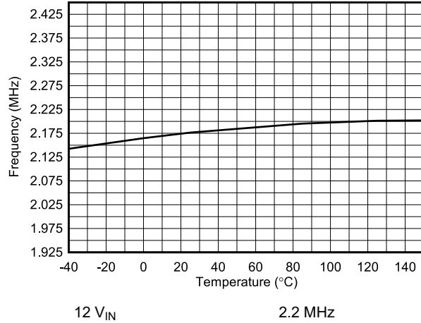
Figure 6-55. Oscillator Frequency vs Temperature
