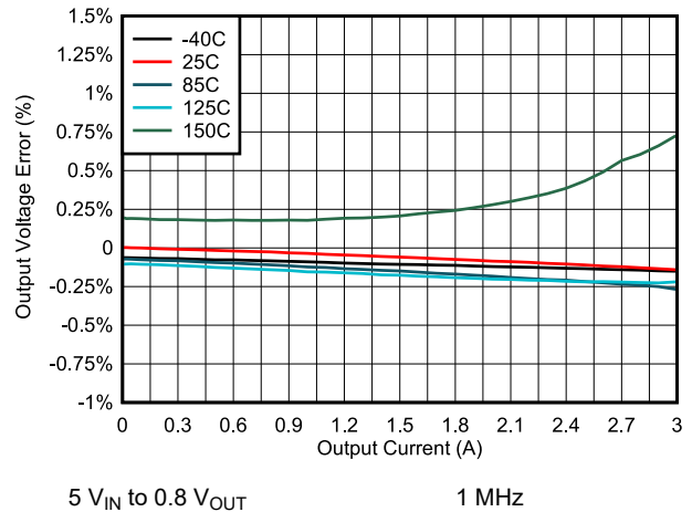
Figure 6-52. Output Voltage Error vs Load
