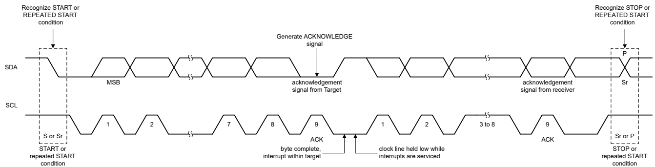
Figure 8-20. Bus Protocol
