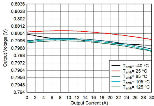
Figure 10-8. Output Voltage vs Output Current
