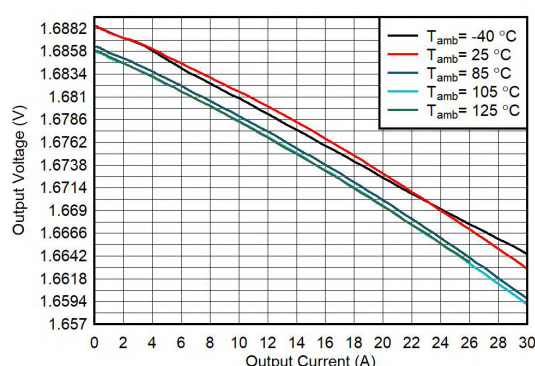
V_{IN} = 3.3V FPWM; TPS6287B25 droop enabled V_{OUT} = 1.675V
