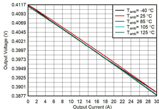
V_{IN} = 3.3V FPWM; TPS6287B25 droop enabled V_{OUT} = 0.4V
