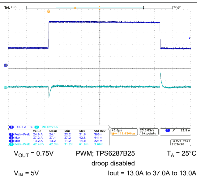
Figure 10-31. Load Transient Response
