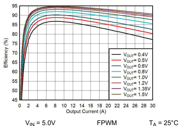
Figure 10-2. Efficiency vs Output Current
