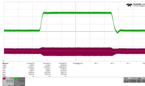
Figure 10-22. Load Transient Response
