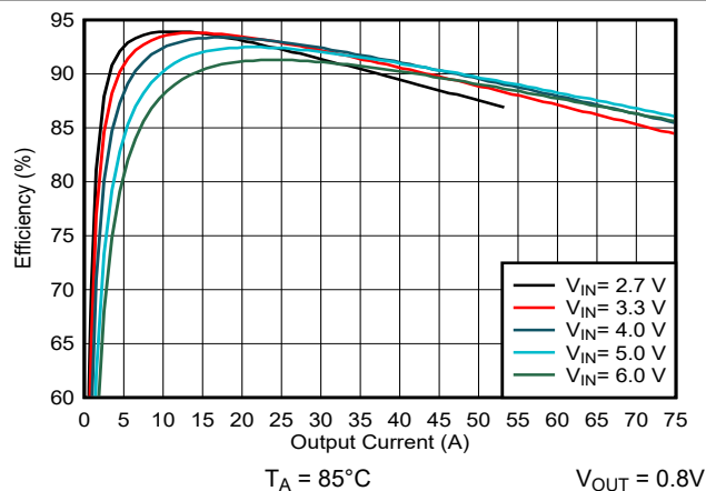
Figure 10-38. Efficiency vs Output Current
