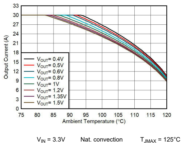
Figure 10-7. Safe Operating Area
