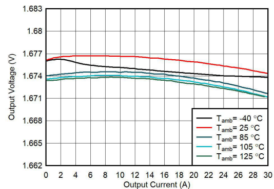
Figure 10-10. Output Voltage vs Output Current
