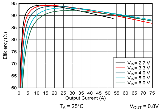
Figure 10-36. Efficiency vs Output Current
