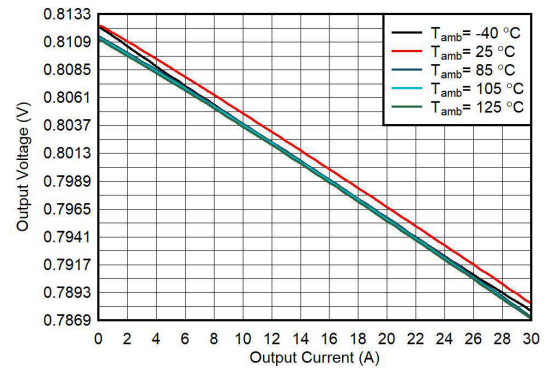
Figure 10-9. Output Voltage vs Output Current
