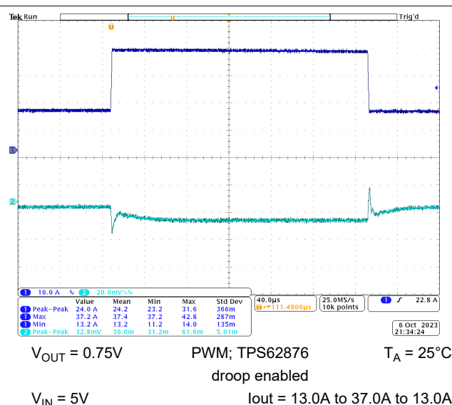
Figure 10-32. Load Transient Response
