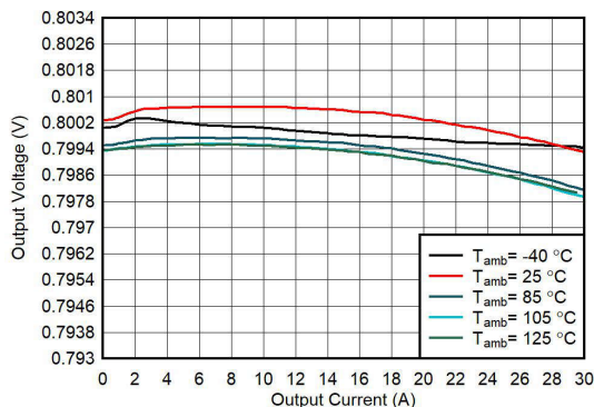
V_{IN} = 3.3V FPWM; TPS6287B25 droop disabled V_{OUT} = 0.8V
