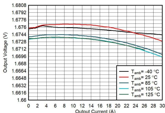
V_{IN} = 3.3V FPWM; TPS6287B25 droop disabled V_{OUT} = 1.675V
