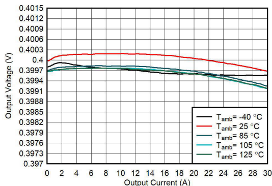
V_{IN} = 3.3V FPWM; TPS6287B25 droop disabled V_{OUT} = 0.4V
