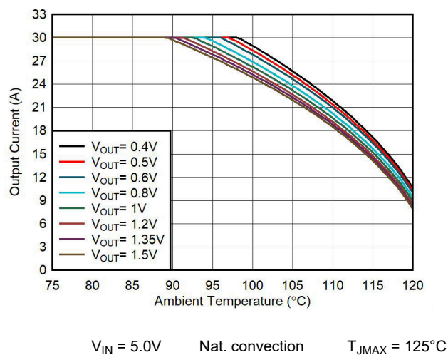
Figure 10-6. Safe Operating Area
