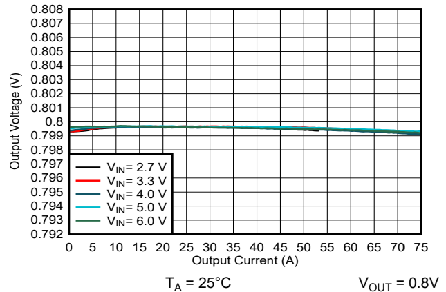
Figure 10-37. Output Voltage vs Output Current
