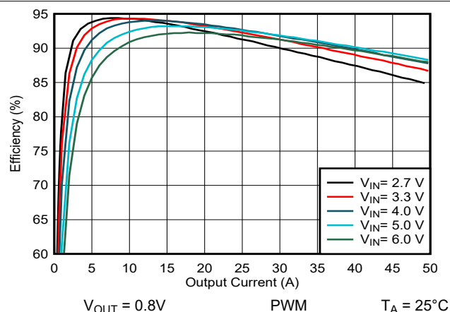
Figure 10-27. Efficiency vs Output Current
