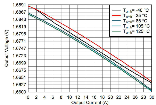
Figure 10-11. Output Voltage vs Output Current
