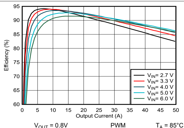
Figure 10-29. Efficiency vs Output Current
