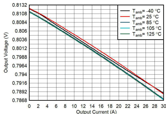
V_{IN} = 3.3V FPWM; TPS6287B25 droop enabled V_{OUT} = 0.8V
