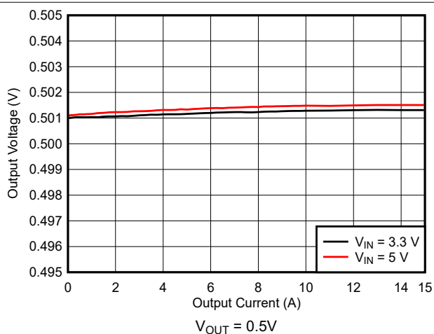
Figure 9-5. Load Regulation
