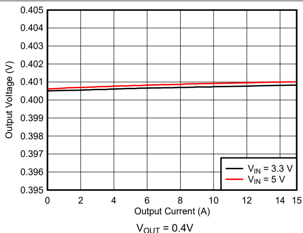
Figure 9-3. Load Regulation
