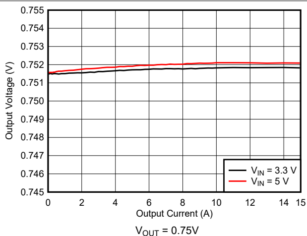
Figure 9-7. Load Regulation
