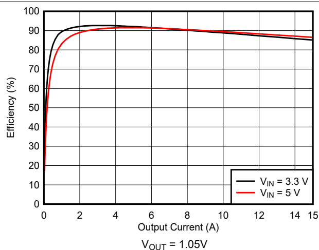
Figure 9-10. Efficiency
