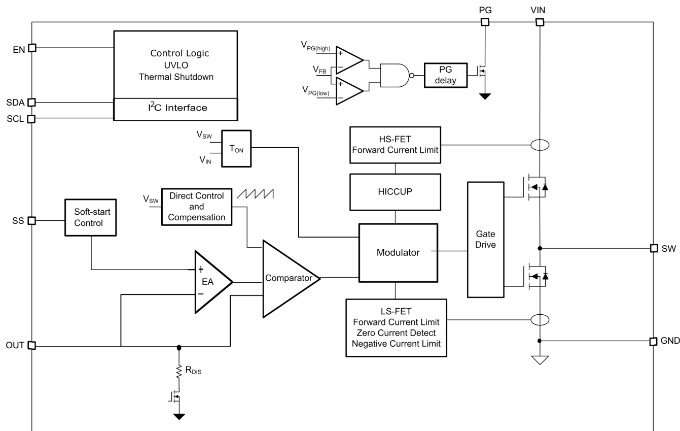
Figure 7-2. Functional Block Diagram - I²C Version (TPS6286Bxx)
