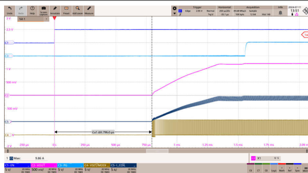
Figure 9-22. FPWM Operation
