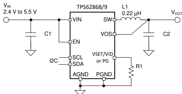
Typical Application
