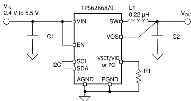
Figure 9-1. Typical Application
