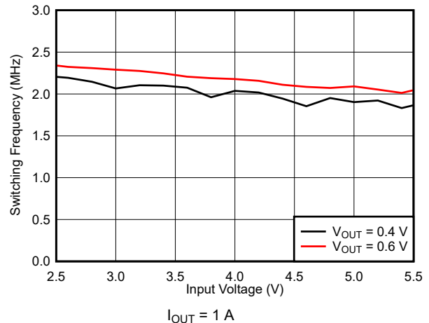
Figure 9-26. Switching Frequency
