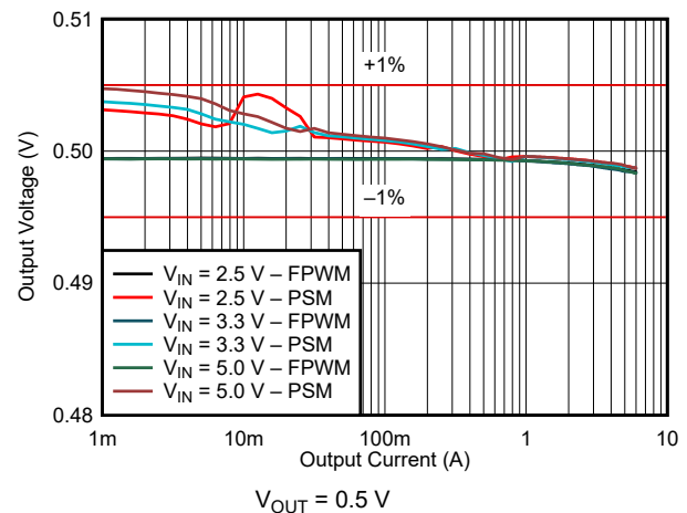
Figure 9-24. Load Regulation
