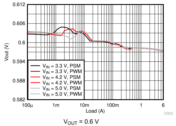
Figure 9-3. Load Regulation
