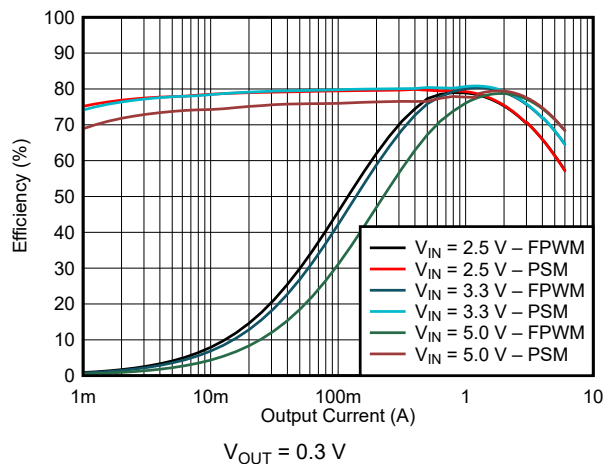
Figure 9-21. Efficiency
