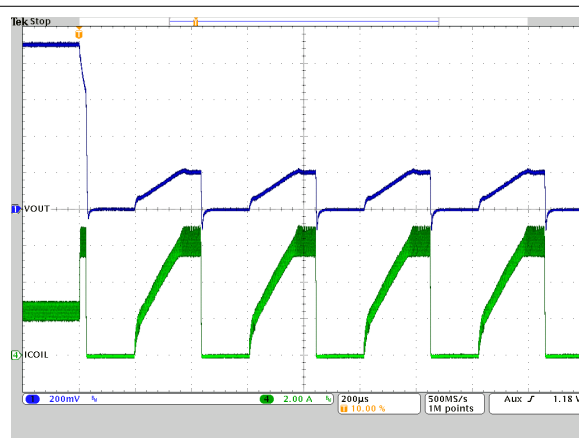
Figure 9-19. HICUP Protection
