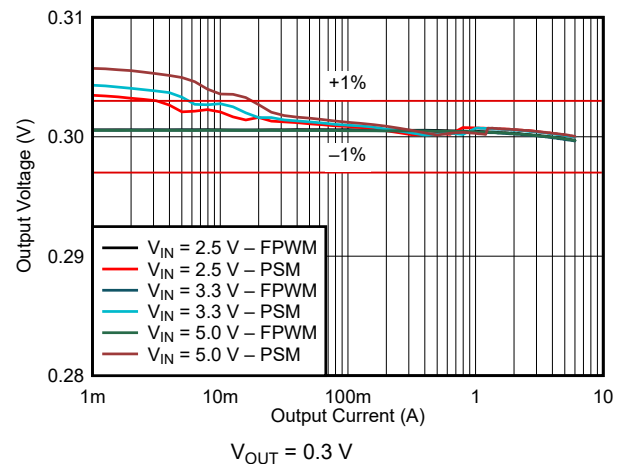
Figure 9-22. Load Regulation
