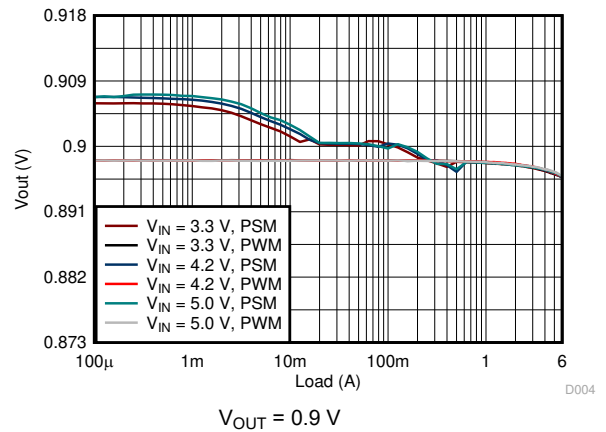
Figure 9-5. Load Regulation
