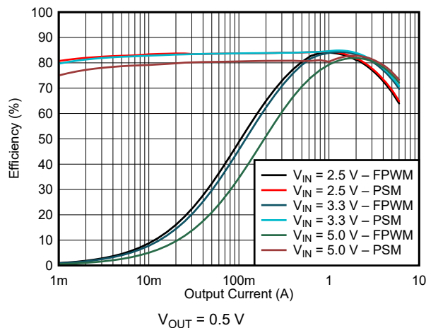
Figure 9-23. Efficiency
