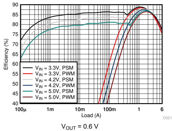
Figure 9-2. Efficiency
