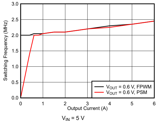
Figure 9-25. Switching Frequency
