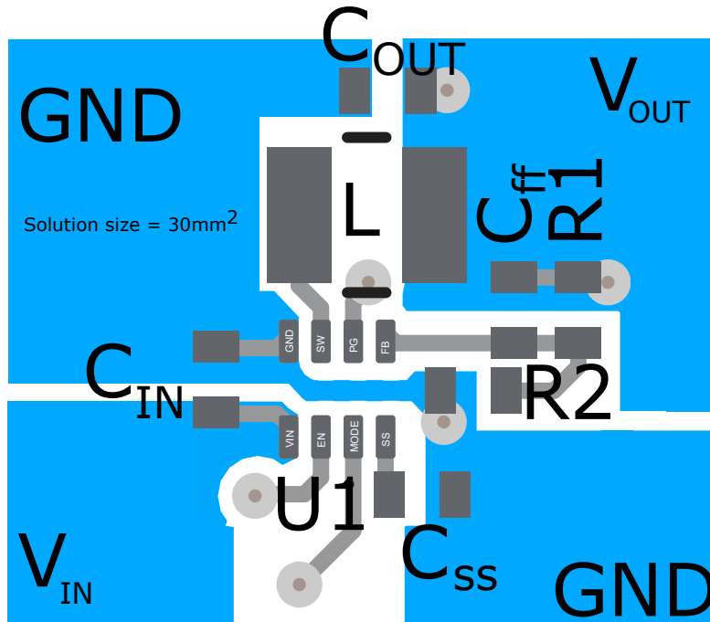
Figure 12-1. Example Layout
