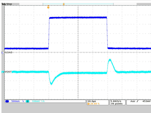
Figure 9-24. Load Transient Response
