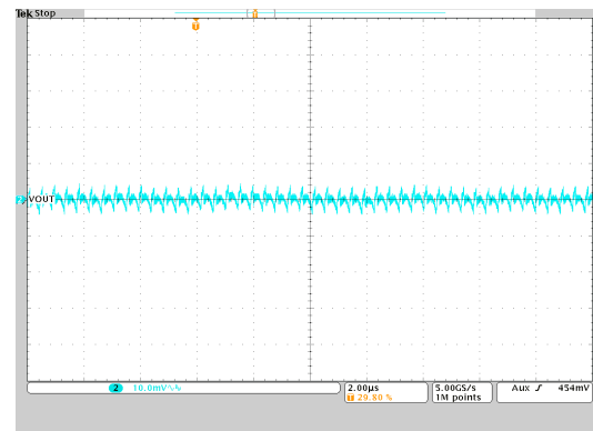
Figure 9-47. Output Voltage Ripple
