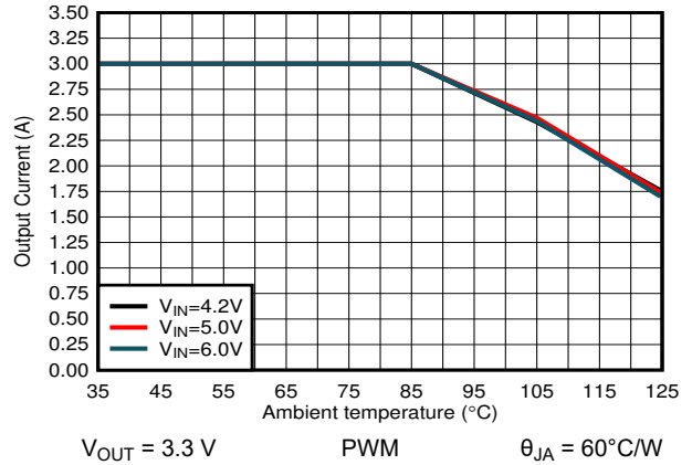
Figure 9-21. Output Current vs Ambient Temperature
