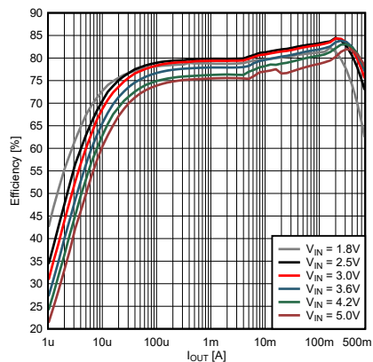
Figure 8-2. Efficiency at V_{OUT} = 0.4V
