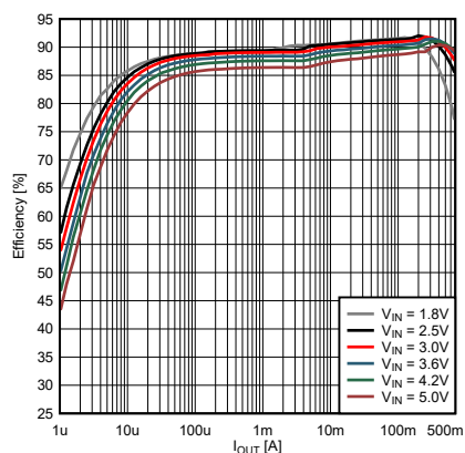
Figure 8-4. Efficiency at V_{OUT} = 1.2V
