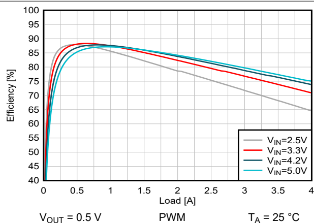
Figure 8-14. Efficiency versus Output Current
