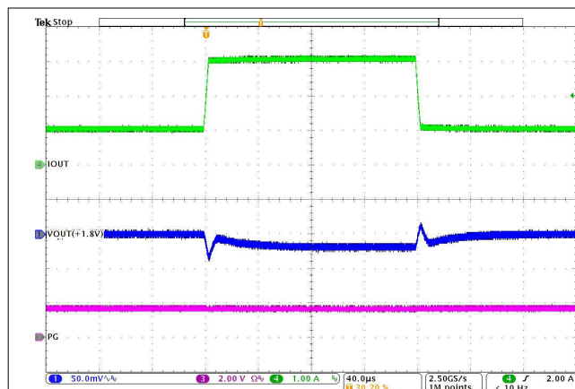
Figure 8-33. Load Transient
