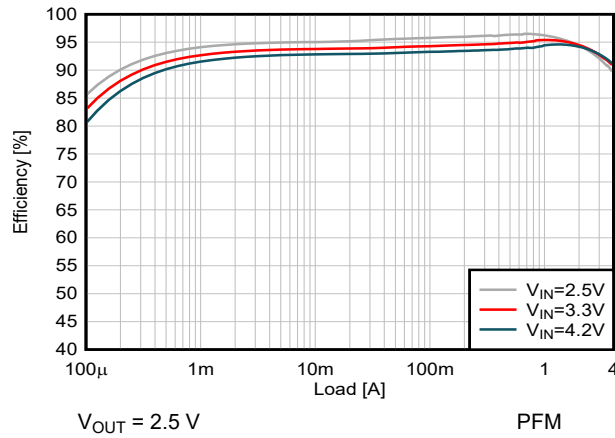
Figure 8-5. Efficiency versus Output Current
