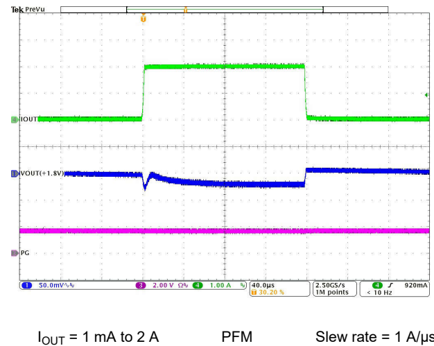
Figure 8-32. Load Transient
