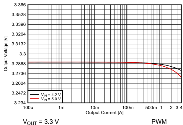
Figure 8-26. Output Voltage versus Output Current
