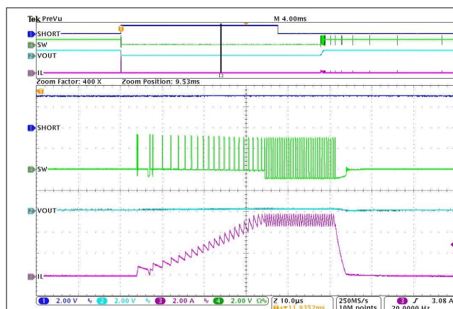
Figure 8-45. HICCUP Short-Circuit Protection (Zoom In - Second Hiccup)
