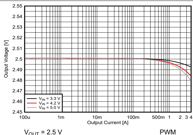
Figure 8-24. Output Voltage versus Output Current
