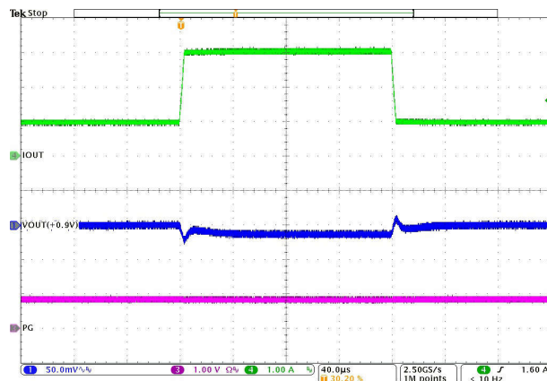
Figure 8-33. Load Transient
