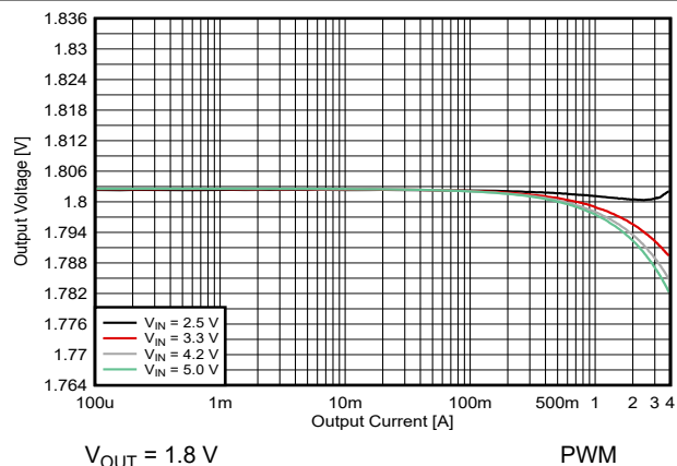
Figure 8-22. Output Voltage versus Output Current
