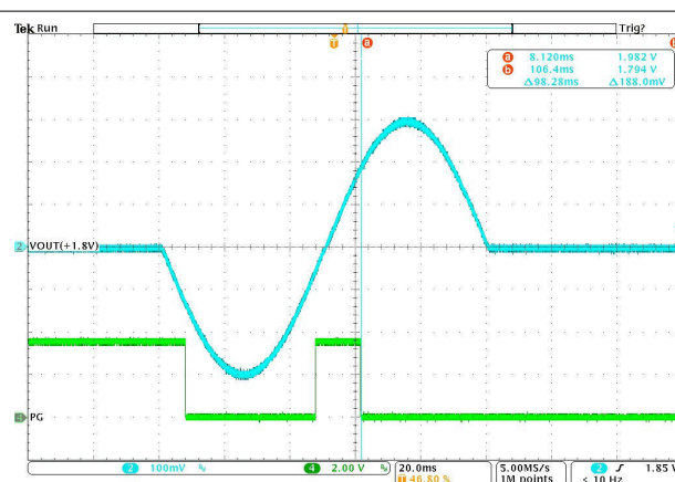
Figure 8-46. Latch-off Short-Circuit Protection
