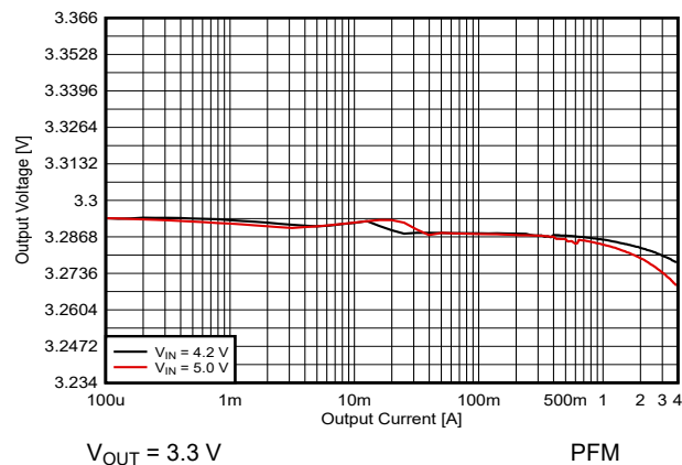
Figure 8-25. Output Voltage versus Output Current
