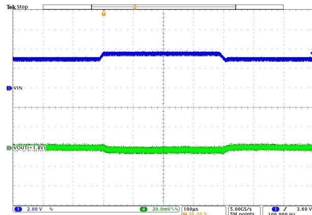
Figure 8-39. Line Transient
