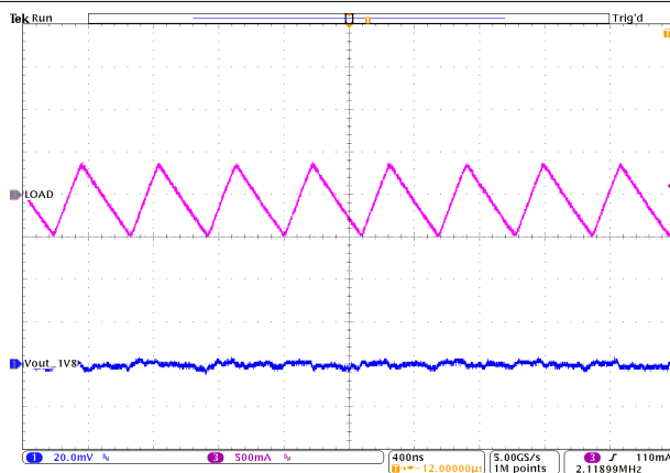
Figure 8-34. PSM Operation
