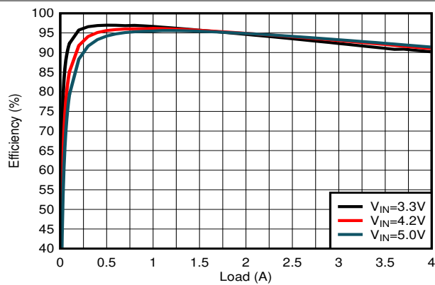
Figure 8-15. Efficiency
