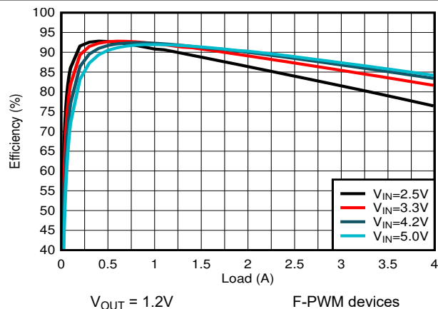
Figure 8-9. PWM Efficiency
