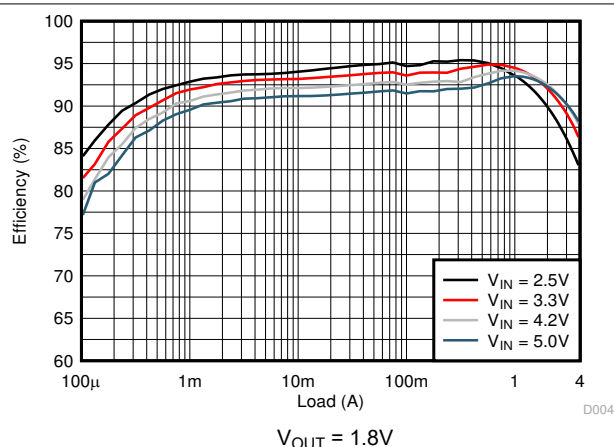
Figure 8-11. Efficiency
