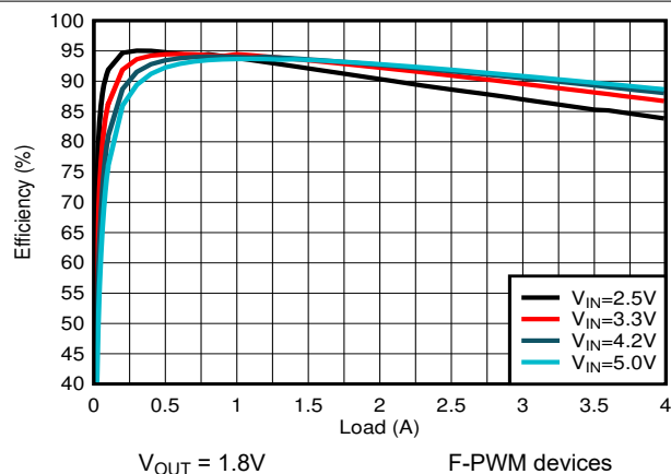
Figure 8-13. PWM Efficiency
