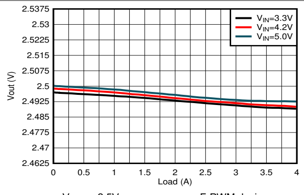
Figure 8-18. Load Regulation
