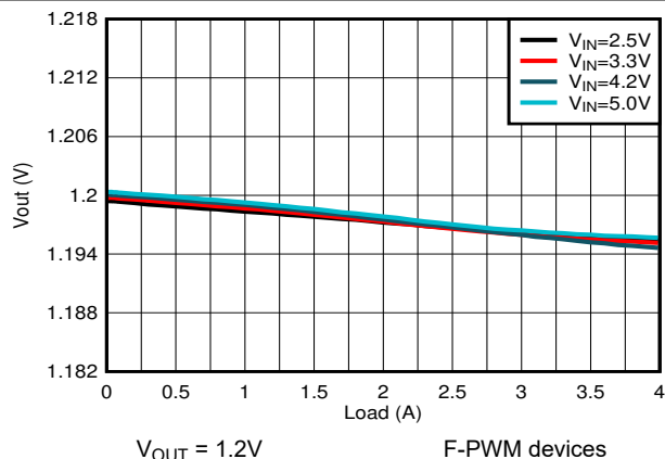
Figure 8-10. Load Regulation
