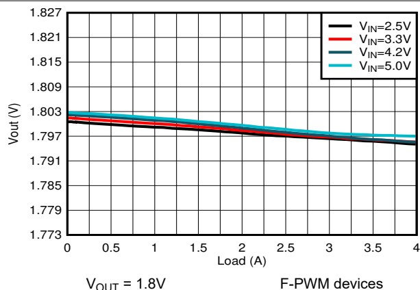
Figure 8-14. Load Regulation
