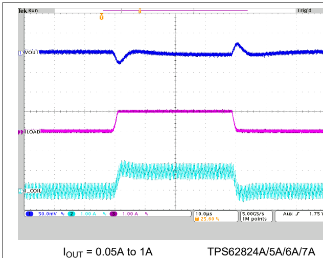
Figure 8-45. Load Transient
