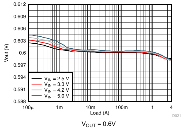
Figure 8-4. Load Regulation
