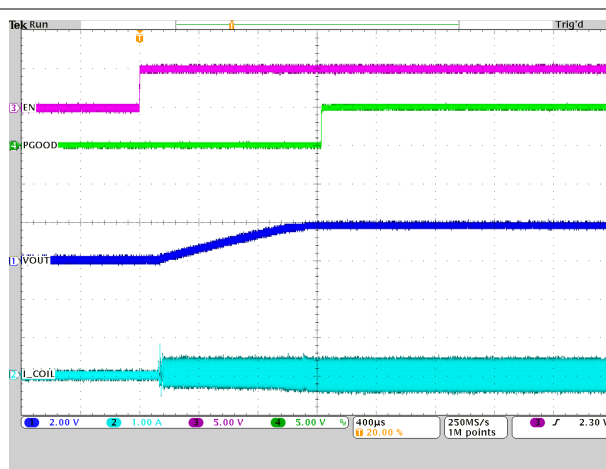
Figure 8-40. Start-Up With No Load
