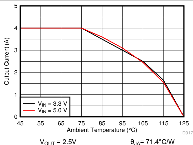
Figure 8-31. Thermal Derating
