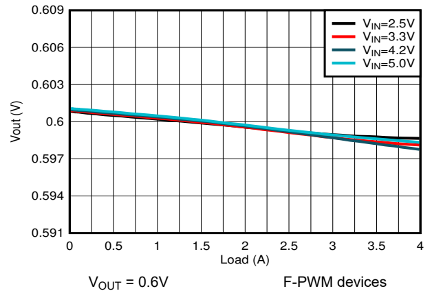
Figure 8-6. Load Regulation
