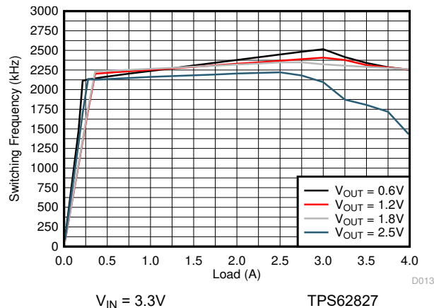
Figure 8-27. Switching Frequency
