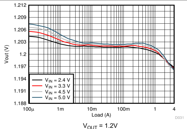
Figure 8-8. Load Regulation
