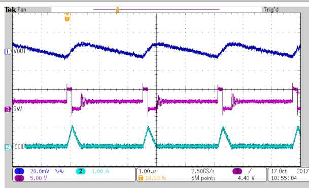
Figure 8-34. PSM Operation
