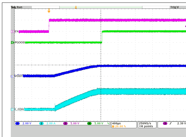
Figure 8-39. Start-Up With Load
