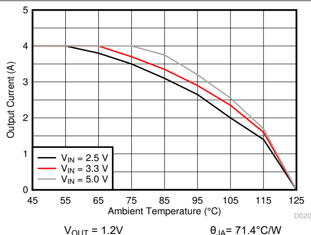
Figure 8-29. Thermal Derating
