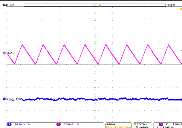
Figure 8-34. PSM Operation
