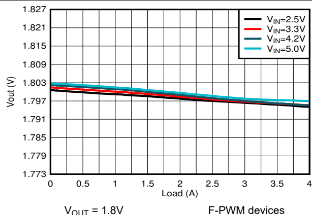
Figure 8-14. Load Regulation
