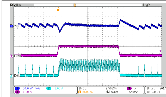
Figure 8-43. Load Transient
