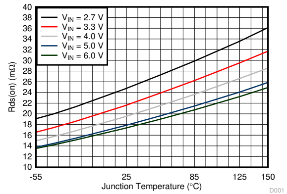
Figure 6-2. R_{ds(on)} of Low-side Switch
