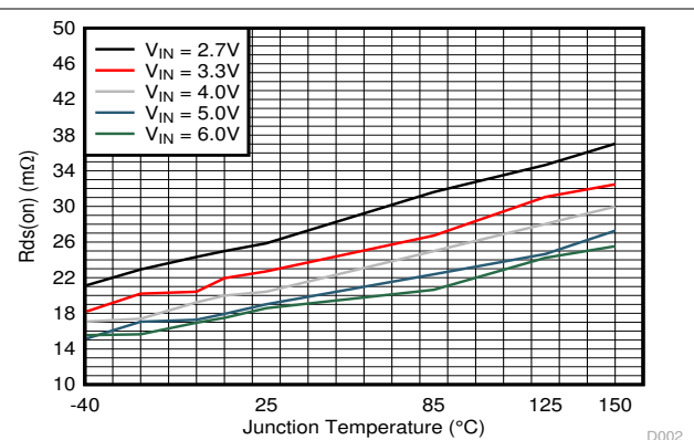
Figure 6-2. R_{ds(on)} of Low-side Switch
