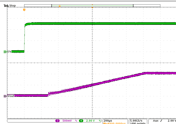
Figure 9-53. Start-Up Timing
