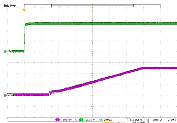
Figure 9-52. Start-Up Timing
