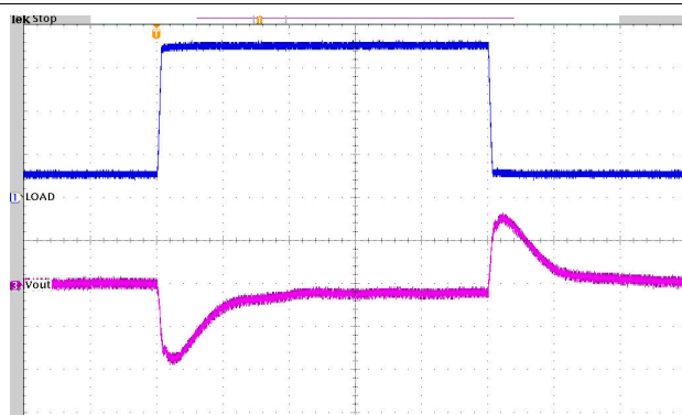
Figure 10-23. Load Transient Response
