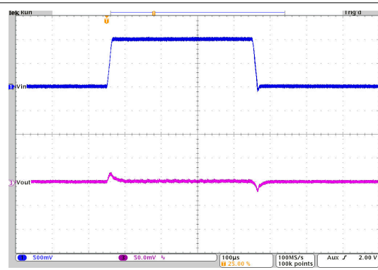
Figure 10-35. Line Transient Response
