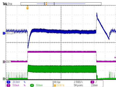
TPS62801 V_{OUT} = 1.2\text{ V} V_{SEL}/\text{MODE} = \text{GND} rise / fall time < 1\text{ }\mu\text{s} PFM / PWM mode I_{OUT} = 5\text{ mA to } 500\text{ mA}
