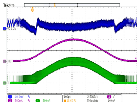
TPS62801 V_{OUT} = 1.2\text{ V} V_{SEL}/\text{MODE} = \text{GND} I_{OUT} = 1\text{ mA to } 1\text{ A } 1\text{ kHz} PFM/PWM mode
