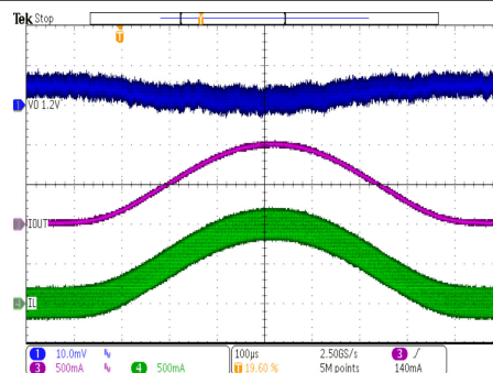
TPS62801 V_{OUT} = 1.2\text{ V} V_{SEL}/\text{MODE} = \text{VIN} I_{OUT} = 1\text{ mA to } 1\text{ A } 1\text{ kHz} (after start-up) Forced PWM mode
