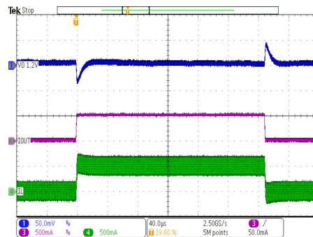
Forced V_{OUT} = 1.2\text{ V} V_{SEL}/\text{MODE} = \text{VIN} PWM mode (after start-up) rise / fall time < 1\text{ }\mu\text{s} I_{OUT} = 5\text{ mA to } 500\text{ mA}
