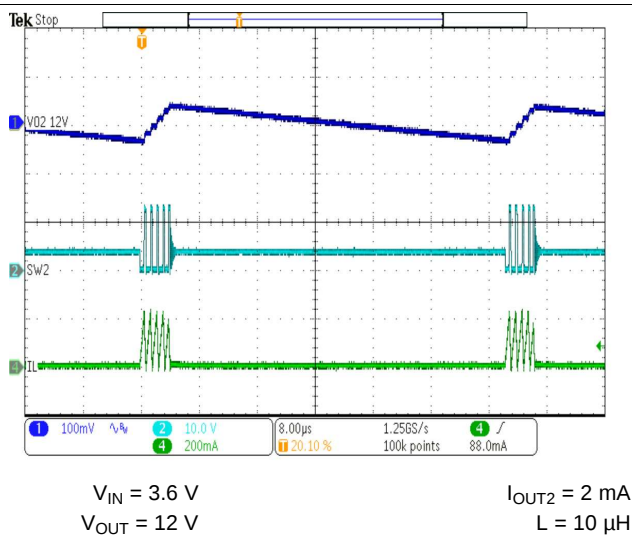
Figure 33. Typical Operation PFM Mode
