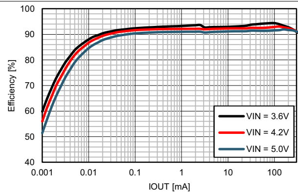
Figure 11. Efficiency vs. IOUT, VOUT1 = 1.2 V
