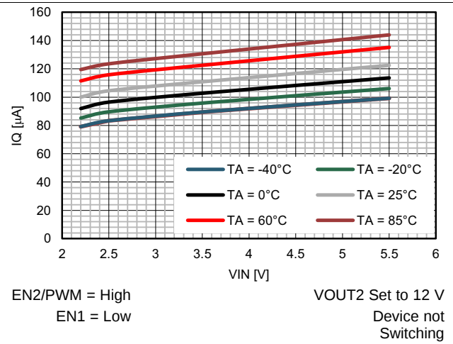
Figure 2. Quiescent Current I_Q Step-Up converter
