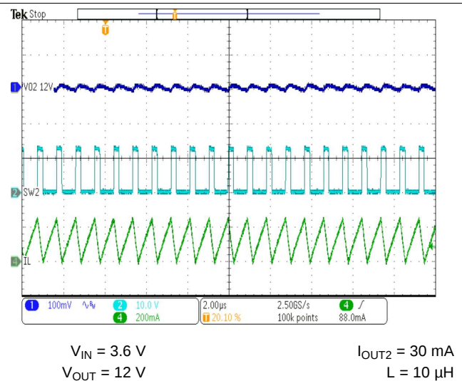
Figure 34. Typical Operation PWM Mode
