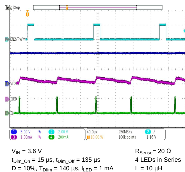
Figure 43. Constant Current with EN2/PWM = 10% D
