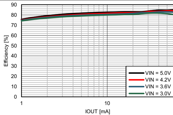
Figure 29. Efficiency vs. IOUT, VOUT = 15 V
