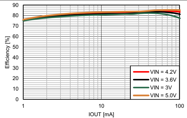
Figure 30. Efficiency vs. IOUT, VOUT = 12 V
