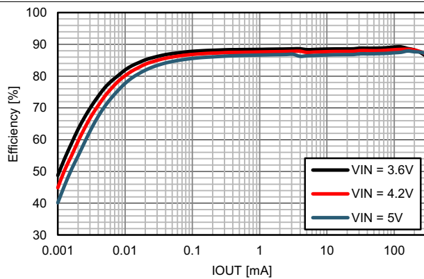
Figure 10. Efficiency vs. IOUT, VOUT1 = 1.0 V
