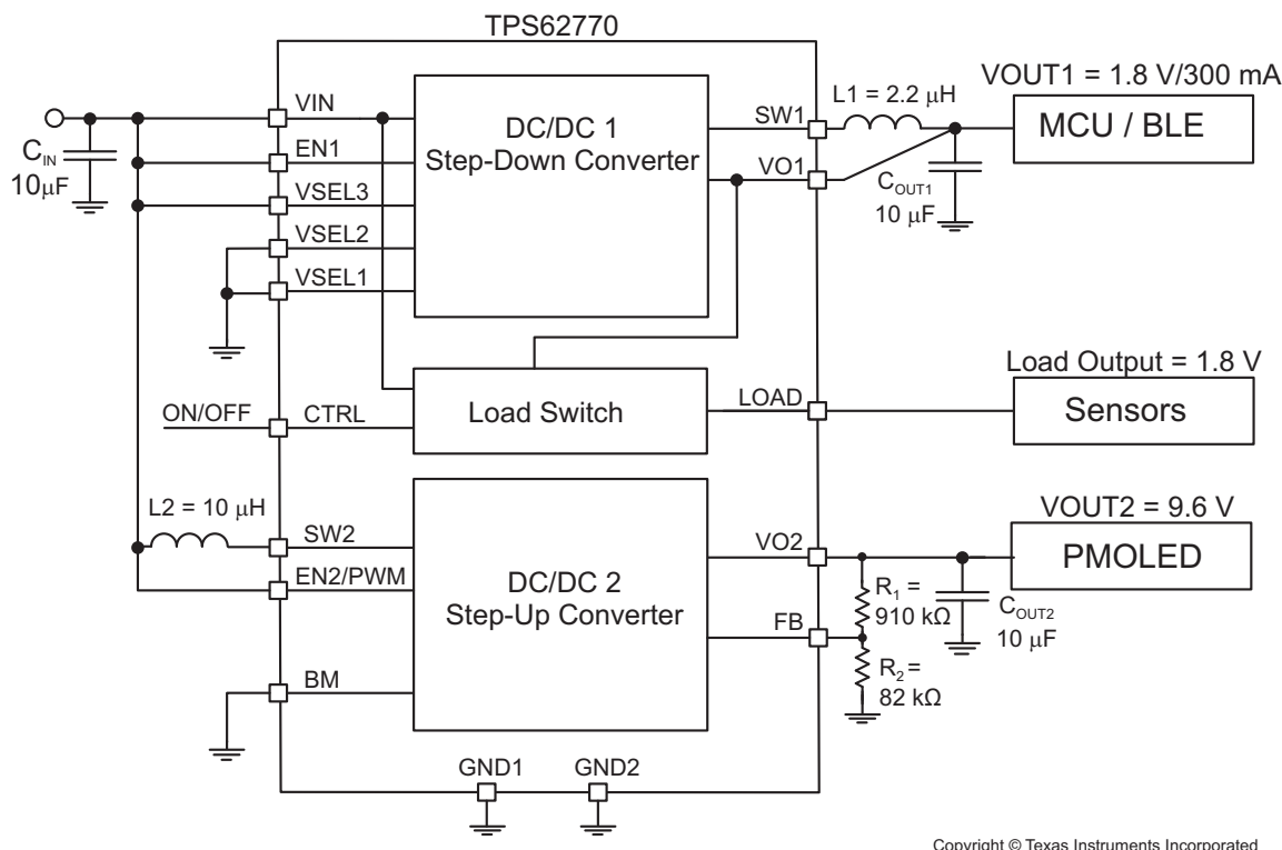
Figure 27. Schematic for Step-Up Converter with Adjustable Output Voltage (9V-15V)
