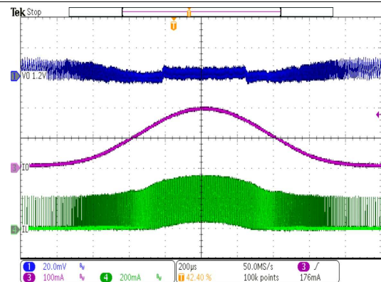
Figure 19. Typical Operation in PWM Mode
