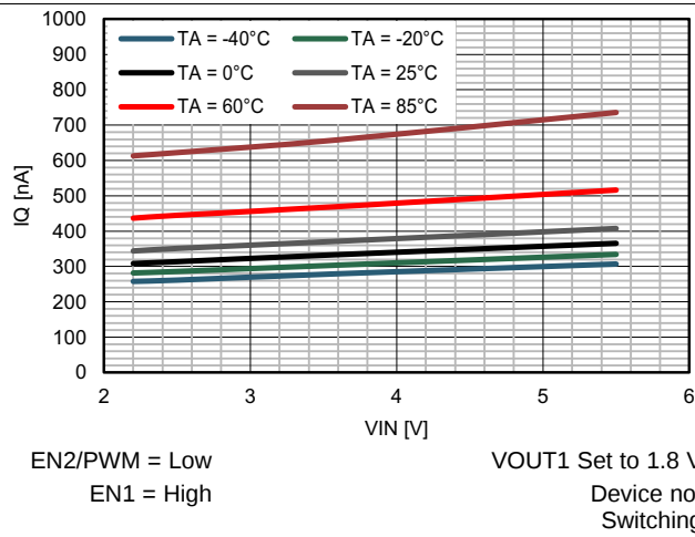
Figure 1. Quiescent Current I_Q Step-Down converter
