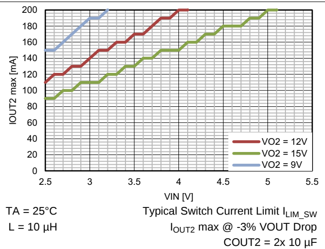
Figure 32. Maximum Output Current vs VIN for Typical I_{LIM\_SW}
