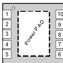
DSK PACKAGE (TOP VIEW)
