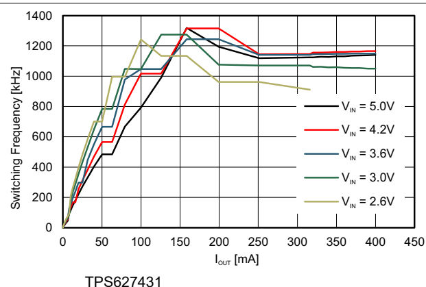
TPS627431 Figure 9-11. Switching Frequency vs Load Current V_{OUT} = 1.4\text{ V}
