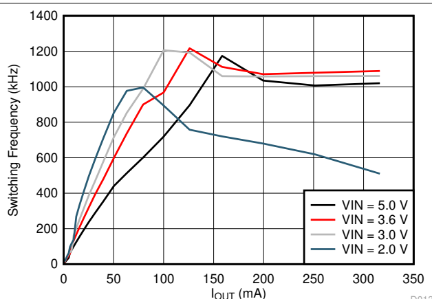
TPS62743 Figure 9-12. Switching Frequency vs Load Current V_{OUT} = 1.2\text{ V}
