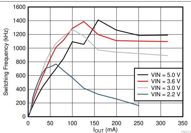
TPS62743 Figure 9-10. Switching Frequency vs Load Current V_{OUT} = 1.8\text{ V}
