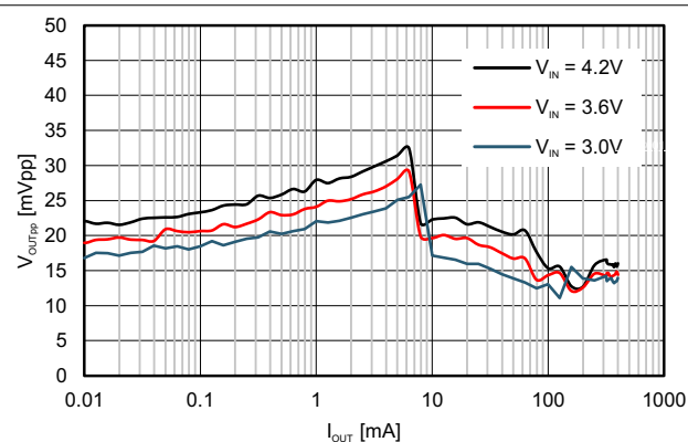
TPS627431 L = 2.2\mu\text{H} C_{OUT} = 10\mu\text{F} (0402) Figure 9-13. Typical Output Ripple Voltage V_{OUT} = 1.4\text{ V}
