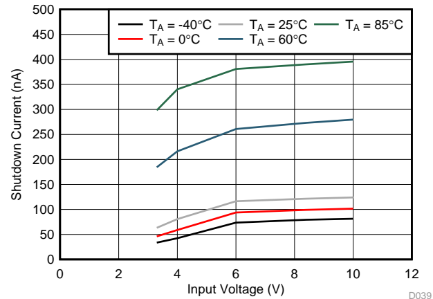
Figure 2. Shutdown Current
