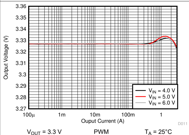
Figure 10-13. Output Voltage vs Output Current
