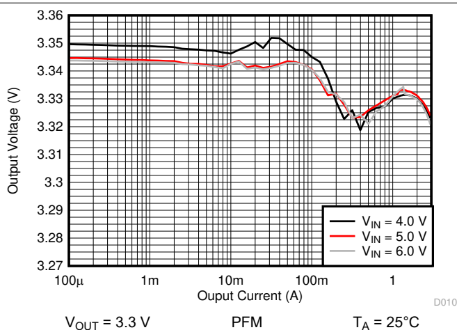
Figure 10-12. Output Voltage vs Output Current
