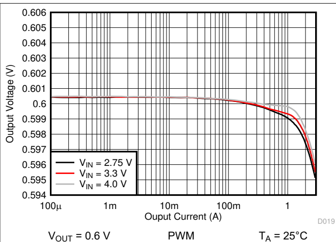
Figure 10-21. Output Voltage vs Output Current
