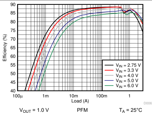
Figure 10-8. Efficiency vs Output Current
