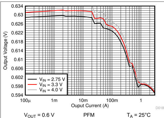
Figure 10-20. Output Voltage vs Output Current
