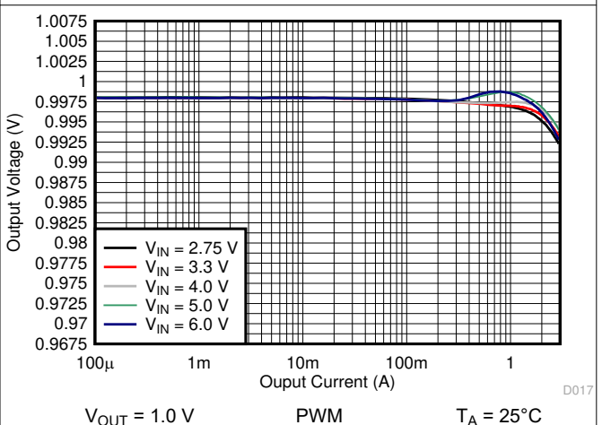
Figure 10-19. Output Voltage vs Output Current
