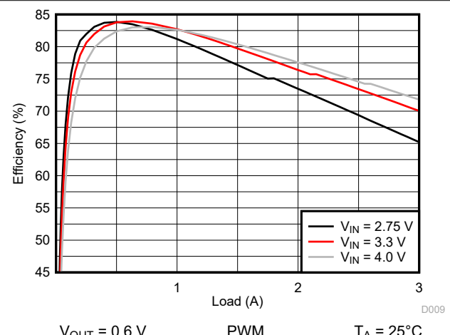
Figure 10-11. Efficiency vs Output Current
