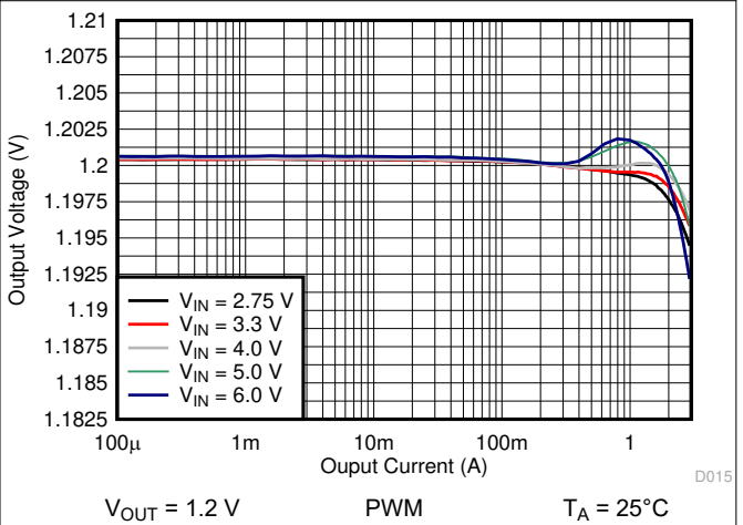
Figure 10-17. Output Voltage vs Output Current
