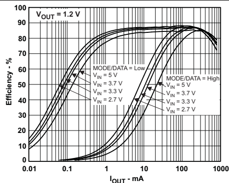
Figure 15. Efficiency V_{OUT} = 1.2\text{ V}
