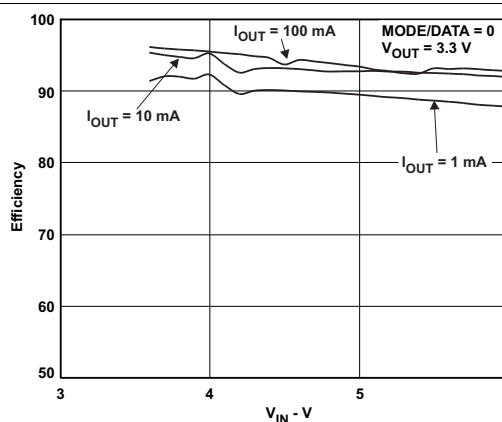
Figure 18. Efficiency V_{OUT} = 3.3\text{ V}
