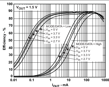
Figure 16. Efficiency V_{OUT} = 1.5\text{ V}
