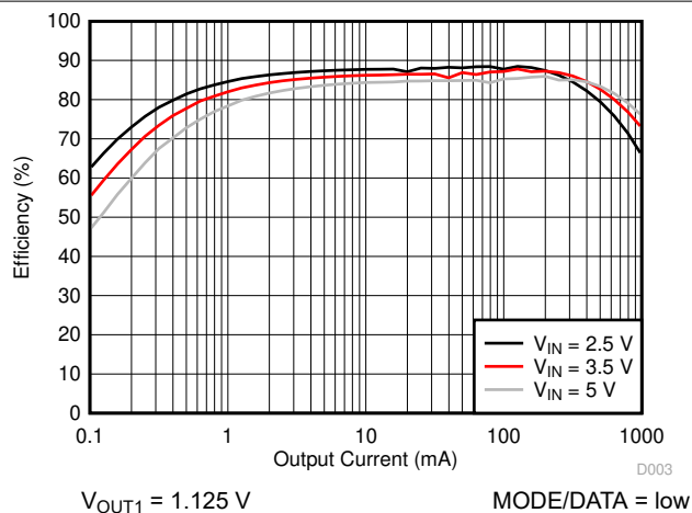
Figure 9-6. TPS62406-Q1 Efficiency, V_{OUT1}
