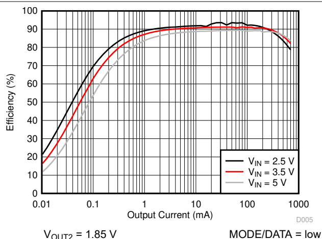
Figure 9-4. TPS62407-Q1 Efficiency, V_{OUT2}
