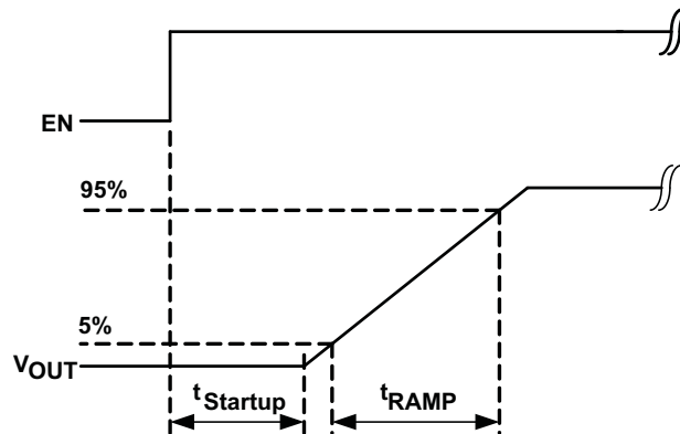
Figure 6. Soft Start
