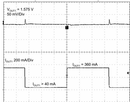
Time base – 50 \mu s/Div PWM mode MODE/DATA = high
