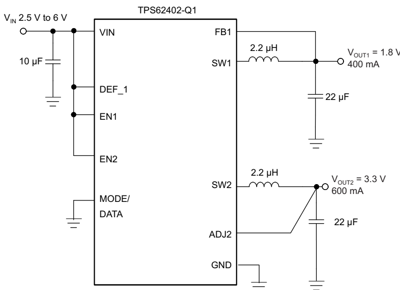
Figure 37. TPS62402-Q1 Fixed 1.8-V and 3.3-V Outputs, Low PFM Ripple Voltage Optimized
