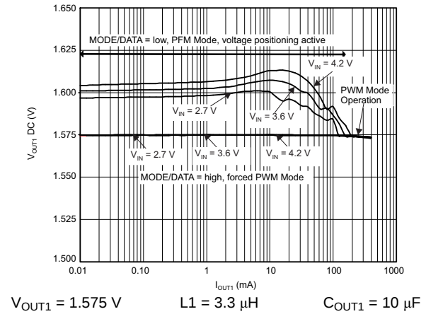
Figure 22. DC Output Accuracy
