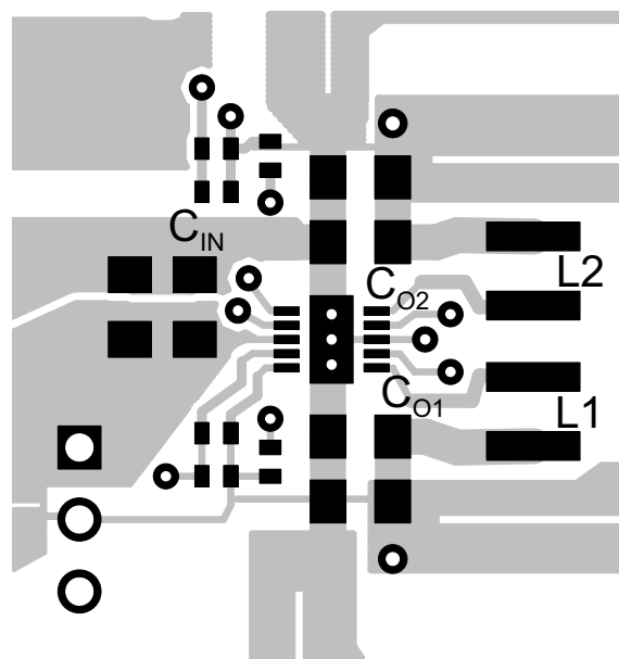
Figure 41. Layout Diagram
