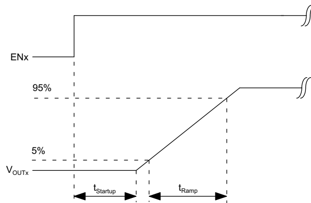
Figure 8. Soft Start
