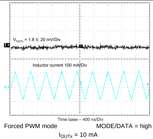
Figure 24. Output-Voltage Ripple in Forced-PWM Mode
